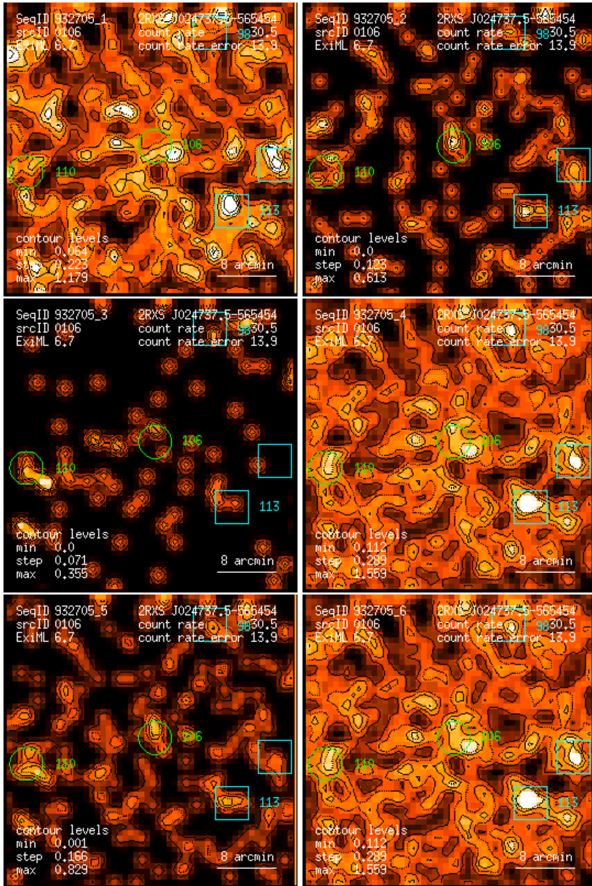
Figure 106: RASS 932705: detection 0106: band rate images, Gaussian filter: (1) PSPC channels 11 – 41, (2) 52 – 90, (3) 91 – 201, (4) 11 – 235, (5) 52 – 201, (6) 11 – 201. Broad band rates in counts/ks. Band rate contour levels in counts/ks/arcmin 2 .
