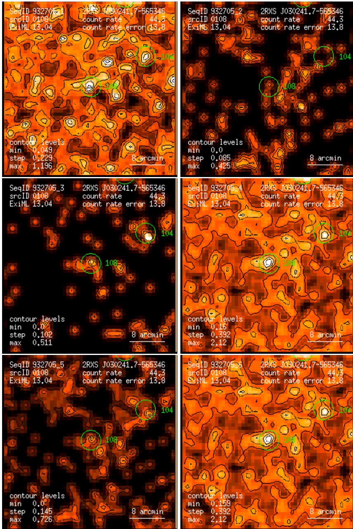
Figure 108: RASS 932705: detection 0108: band rate images, Gaussian filter: (1) PSPC channels 11 – 41, (2) 52 – 90, (3) 91 – 201, (4) 11 – 235, (5) 52 – 201, (6) 11 – 201. Broad band rates in counts/ks. Band rate contour levels in counts/ks/arcmin 2 .
