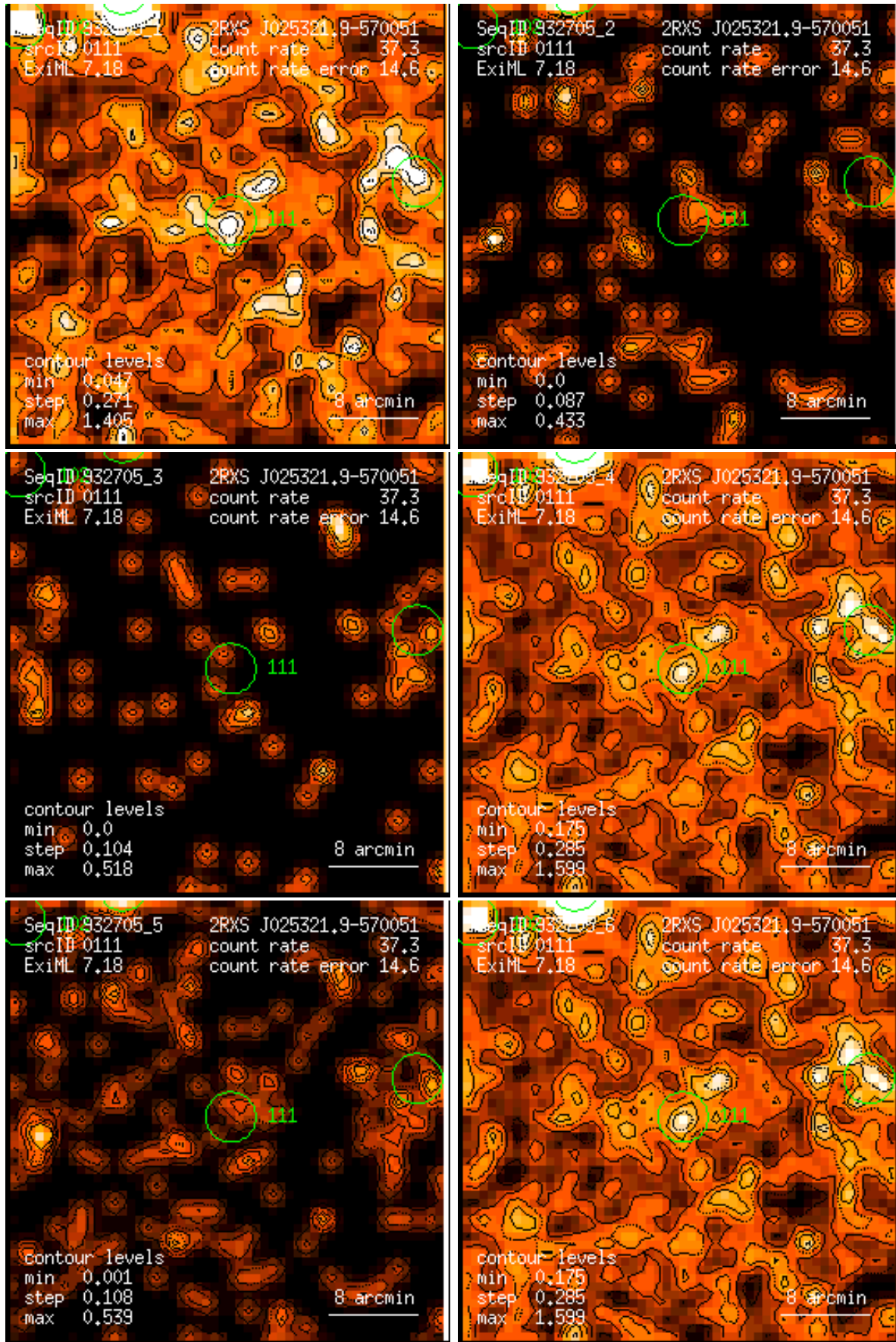
Figure 111: RASS 932705: detection 0111: band rate images, Gaussian filter: (1) PSPC channels 11 – 41, (2) 52 – 90, (3) 91 – 201, (4) 11 – 235, (5) 52 – 201, (6) 11 – 201. Broad band rates in counts/ks. Band rate contour levels in counts/ks/arcmin 2 .
