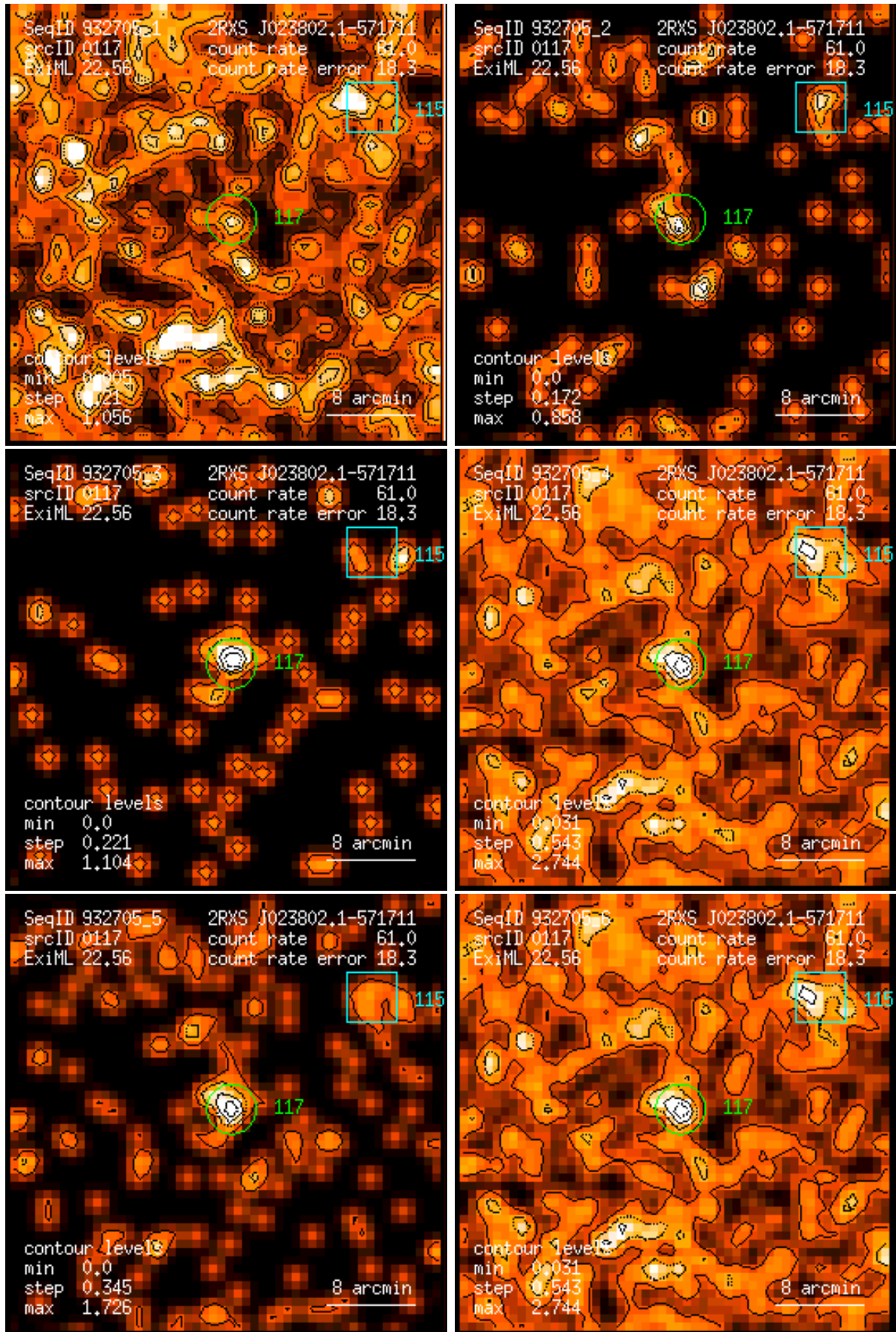
Figure 117: RASS 932705: detection 0117: band rate images, Gaussian filter: (1) PSPC channels 11 – 41, (2) 52 – 90, (3) 91 – 201, (4) 11 – 235, (5) 52 – 201, (6) 11 – 201. Broad band rates in counts/ks. Band rate contour levels in counts/ks/arcmin 2 .
