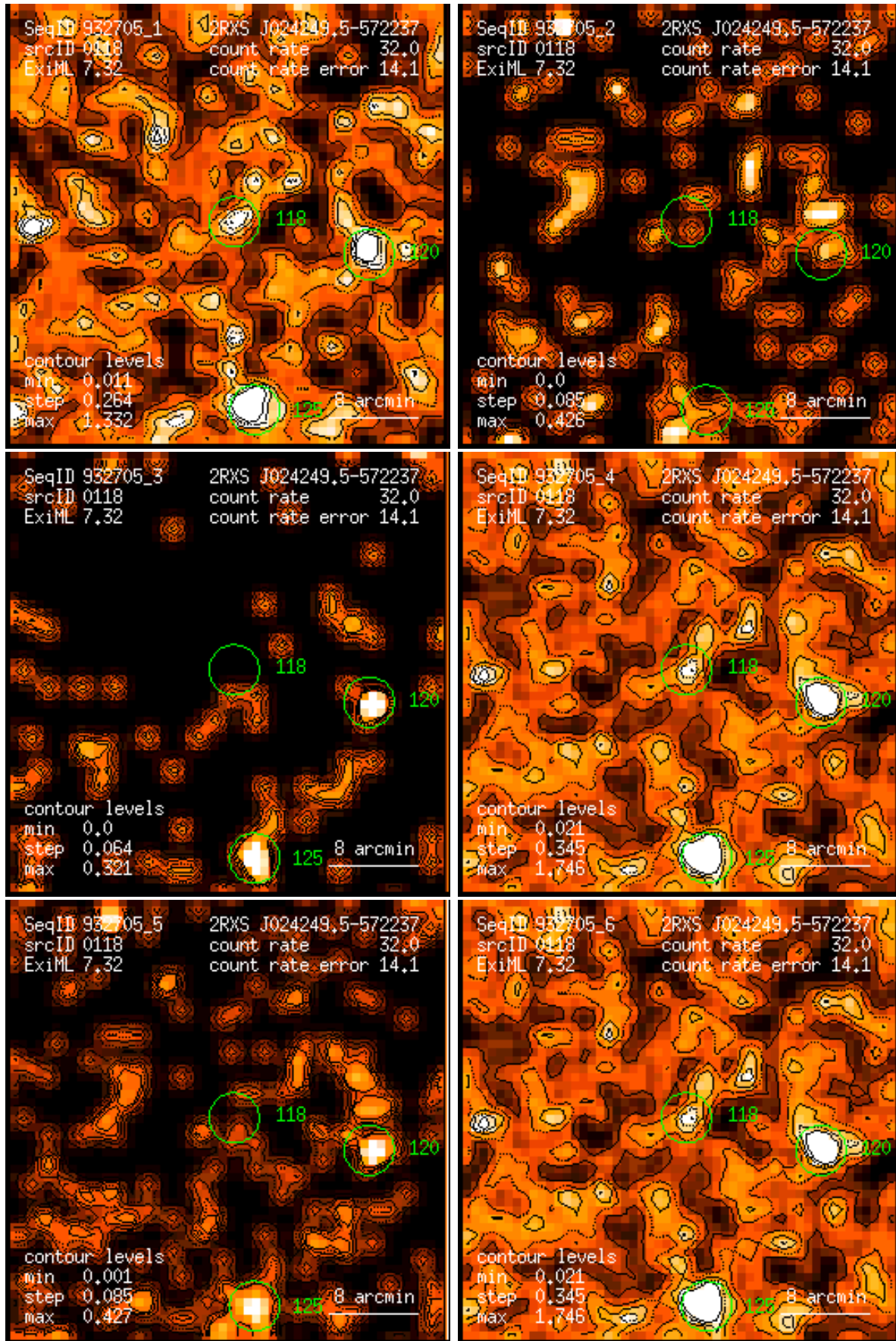
Figure 118: RASS 932705: detection 0118: band rate images, Gaussian filter: (1) PSPC channels 11 – 41, (2) 52 – 90, (3) 91 – 201, (4) 11 – 235, (5) 52 – 201, (6) 11 – 201. Broad band rates in counts/ks. Band rate contour levels in counts/ks/arcmin 2 .
