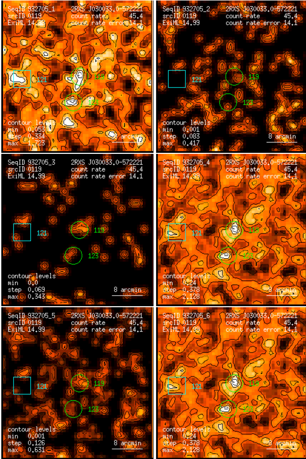
Figure 119: RASS 932705: detection 0119: band rate images, Gaussian filter: (1) PSPC channels 11 – 41, (2) 52 – 90, (3) 91 – 201, (4) 11 – 235, (5) 52 – 201, (6) 11 – 201. Broad band rates in counts/ks. Band rate contour levels in counts/ks/arcmin 2 .
