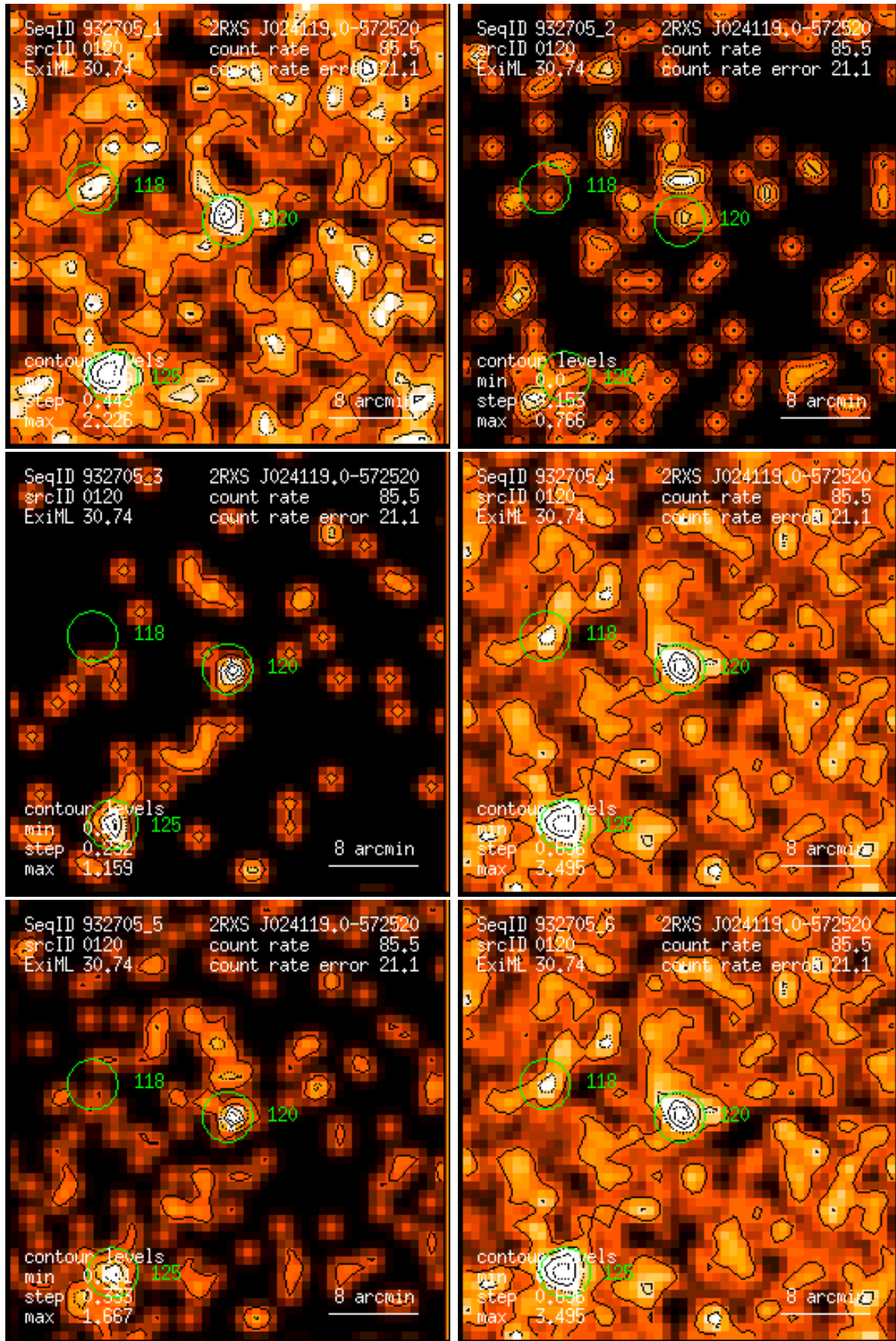
Figure 120: RASS 932705: detection 0120: band rate images, Gaussian filter: (1) PSPC channels 11 – 41, (2) 52 – 90, (3) 91 – 201, (4) 11 – 235, (5) 52 – 201, (6) 11 – 201. Broad band rates in counts/ks. Band rate contour levels in counts/ks/arcmin 2 .
