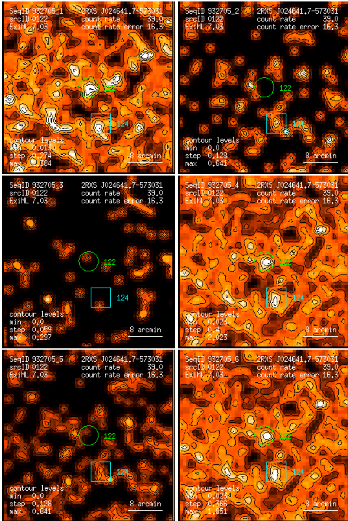
Figure 122: RASS 932705: detection 0122: band rate images, Gaussian filter: (1) PSPC channels 11 – 41, (2) 52 – 90, (3) 91 – 201, (4) 11 – 235, (5) 52 – 201, (6) 11 – 201. Broad band rates in counts/ks. Band rate contour levels in counts/ks/arcmin 2 .
