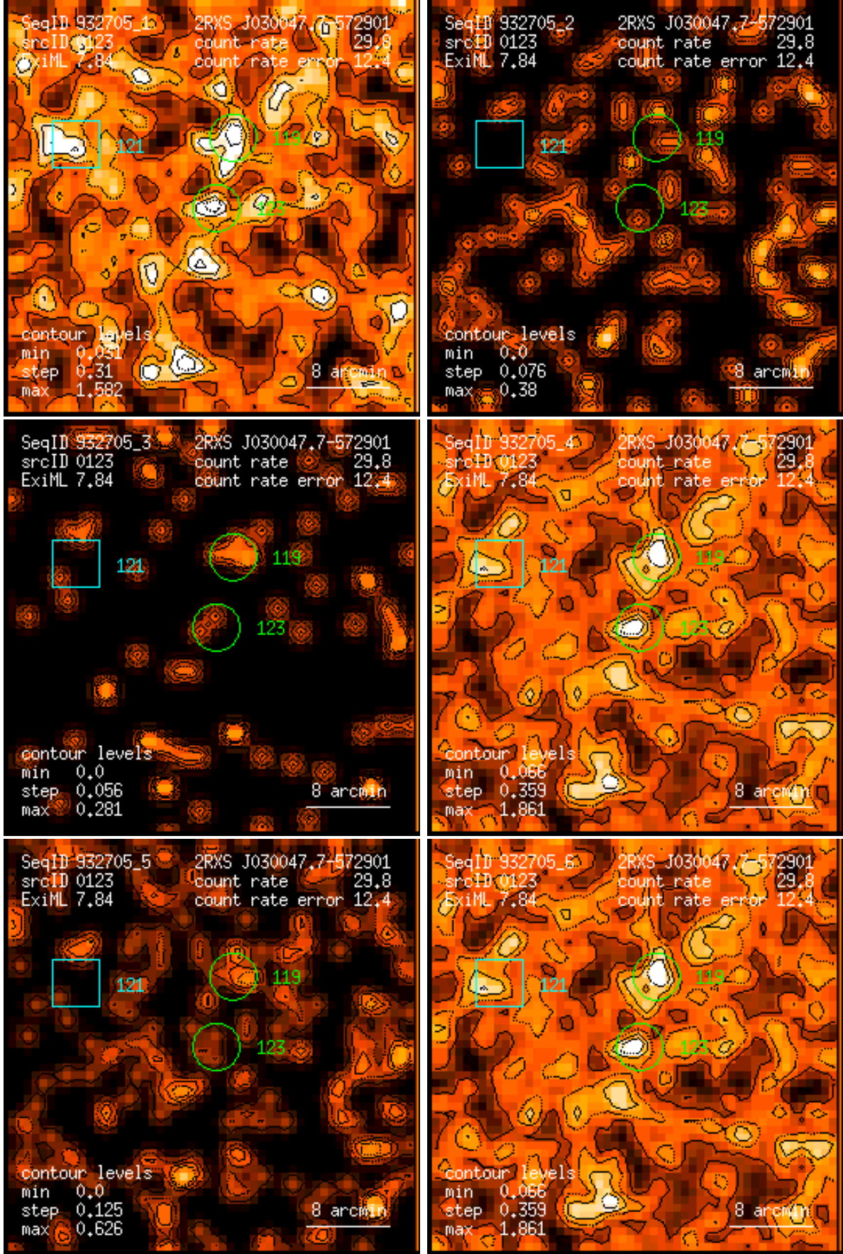
Figure 123: RASS 932705: detection 0123: band rate images, Gaussian filter: (1) PSPC channels 11 – 41, (2) 52 – 90, (3) 91 – 201, (4) 11 – 235, (5) 52 – 201, (6) 11 – 201. Broad band rates in counts/ks. Band rate contour levels in counts/ks/arcmin 2 .
