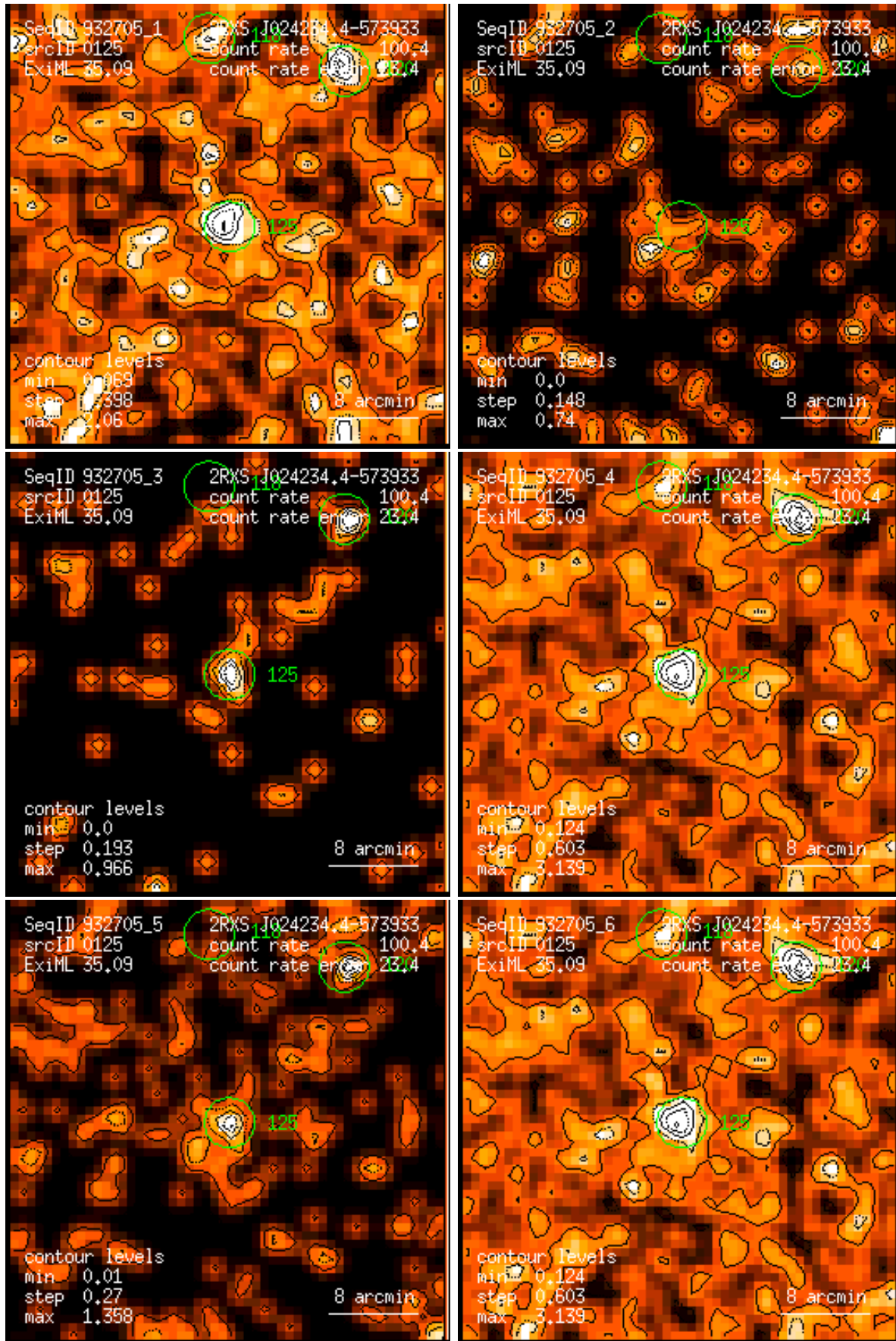
Figure 125: RASS 932705: detection 0125: band rate images, Gaussian filter: (1) PSPC channels 11 – 41, (2) 52 – 90, (3) 91 – 201, (4) 11 – 235, (5) 52 – 201, (6) 11 – 201. Broad band rates in counts/ks. Band rate contour levels in counts/ks/arcmin 2 .
