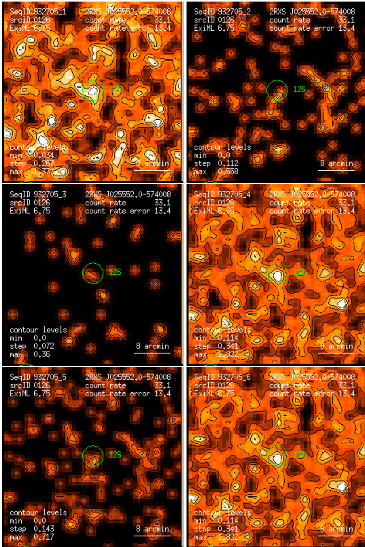
Figure 126: RASS 932705: detection 0126: band rate images, Gaussian filter: (1) PSPC channels 11 – 41, (2) 52 – 90, (3) 91 – 201, (4) 11 – 235, (5) 52 – 201, (6) 11 – 201. Broad band rates in counts/ks. Band rate contour levels in counts/ks/arcmin 2 .
