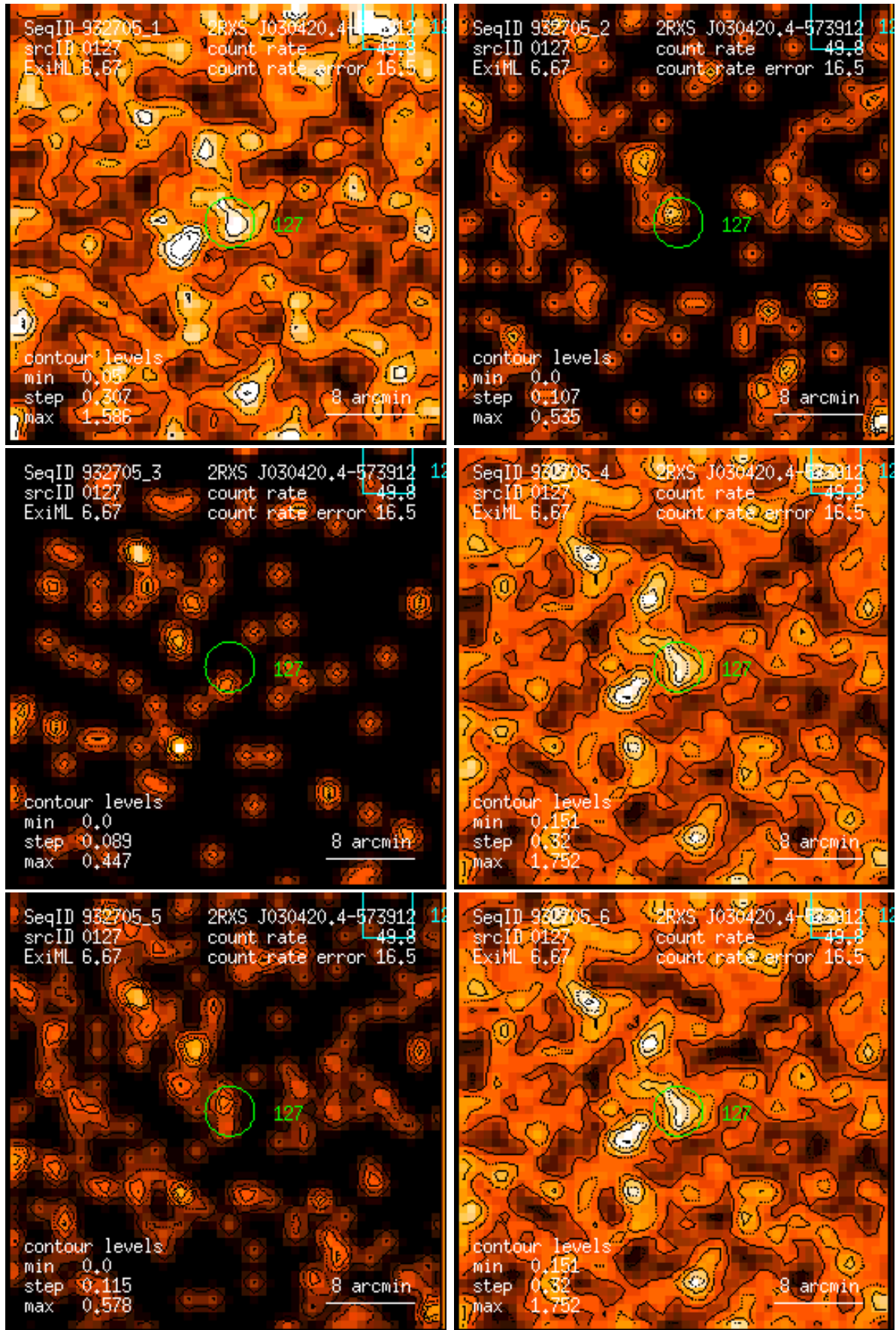
Figure 127: RASS 932705: detection 0127: band rate images, Gaussian filter: (1) PSPC channels 11 – 41, (2) 52 – 90, (3) 91 – 201, (4) 11 – 235, (5) 52 – 201, (6) 11 – 201. Broad band rates in counts/ks. Band rate contour levels in counts/ks/arcmin 2 .
