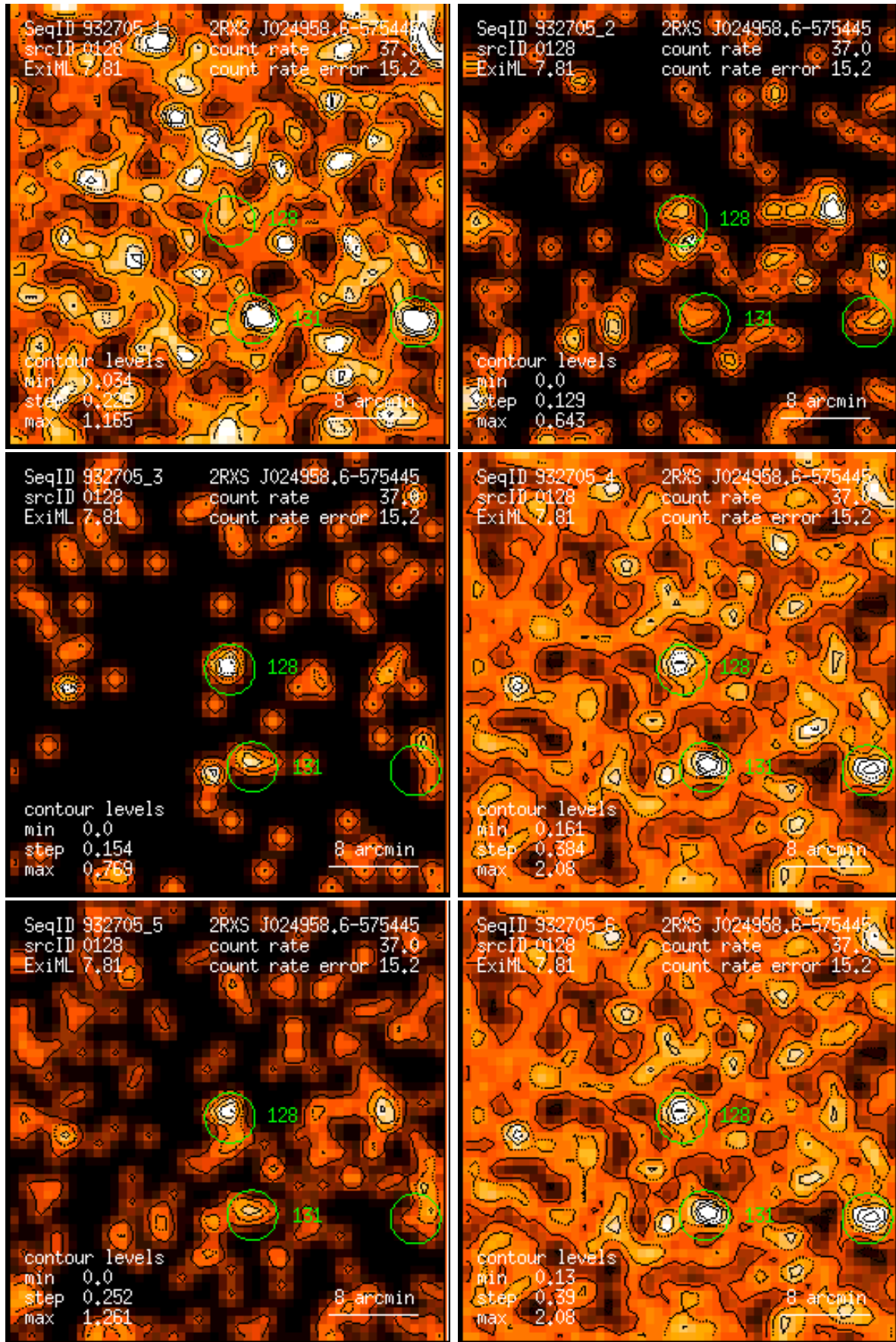
Figure 128: RASS 932705: detection 0128: band rate images, Gaussian filter: (1) PSPC channels 11 – 41, (2) 52 – 90, (3) 91 – 201, (4) 11 – 235, (5) 52 – 201, (6) 11 – 201. Broad band rates in counts/ks. Band rate contour levels in counts/ks/arcmin 2 .
