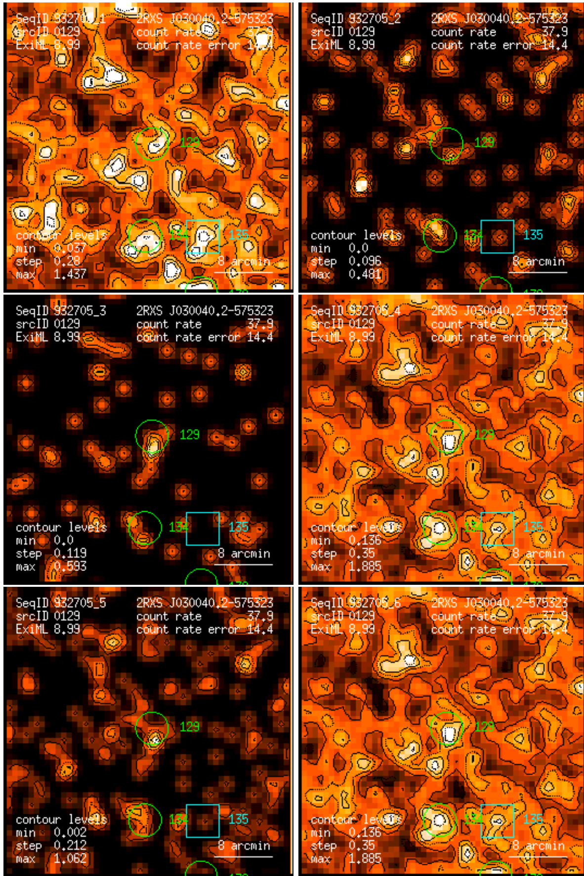
Figure 129: RASS 932705: detection 0129: band rate images, Gaussian filter: (1) PSPC channels 11 – 41, (2) 52 – 90, (3) 91 – 201, (4) 11 – 235, (5) 52 – 201, (6) 11 – 201. Broad band rates in counts/ks. Band rate contour levels in counts/ks/arcmin 2 .
