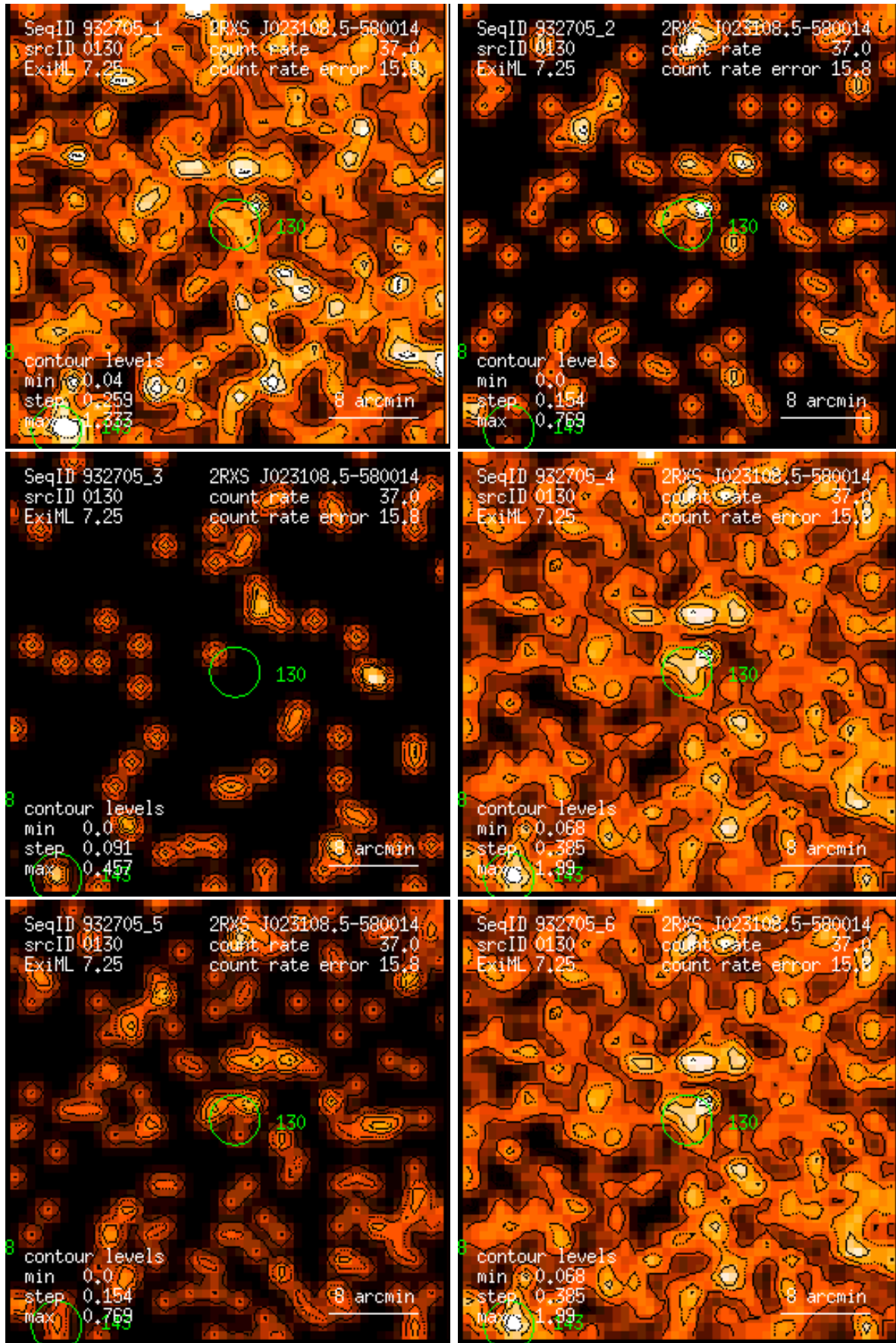
Figure 130: RASS 932705: detection 0130: band rate images, Gaussian filter: (1) PSPC channels 11 – 41, (2) 52 – 90, (3) 91 – 201, (4) 11 – 235, (5) 52 – 201, (6) 11 – 201. Broad band rates in counts/ks. Band rate contour levels in counts/ks/arcmin 2 .
