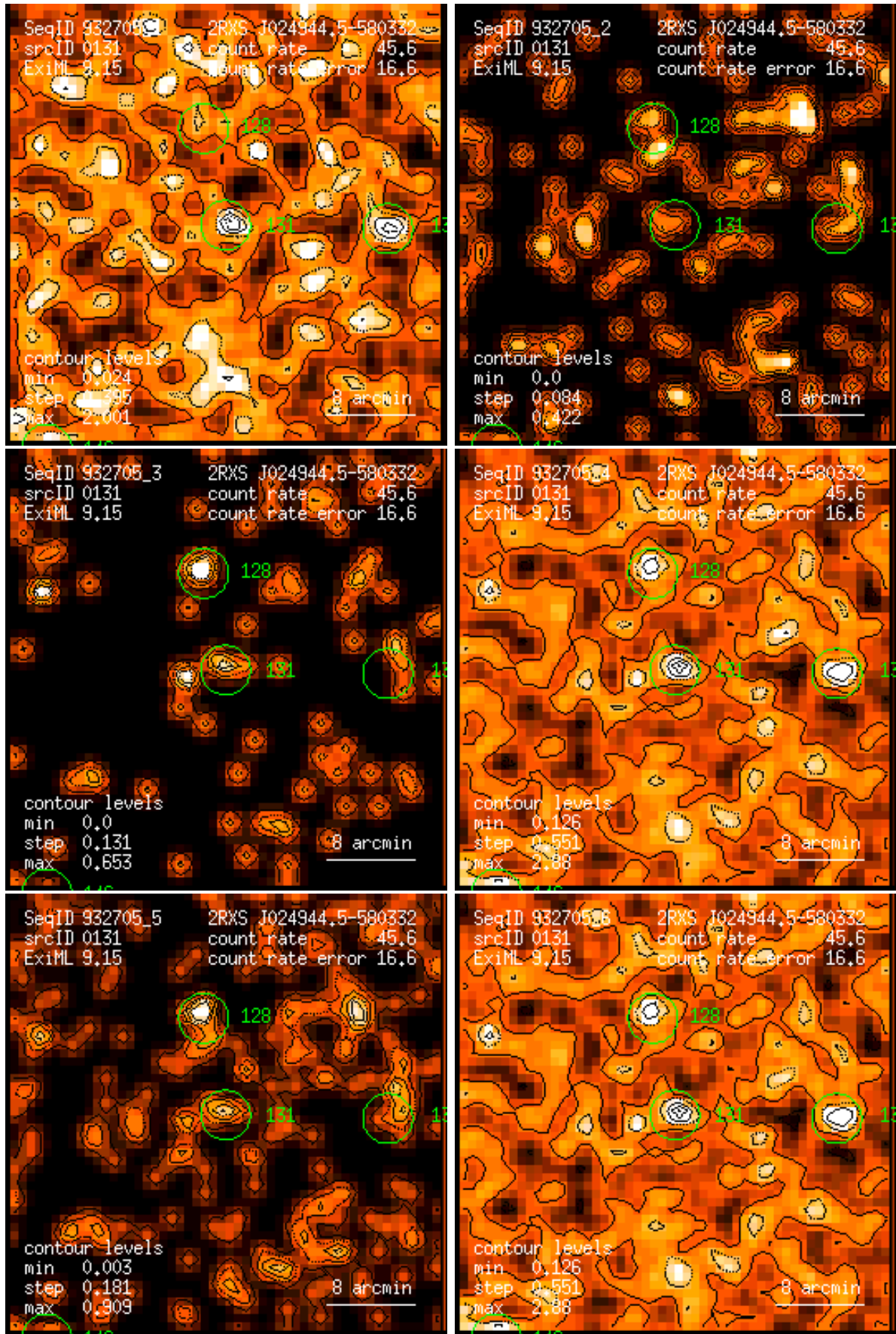
Figure 131: RASS 932705: detection 0131: band rate images, Gaussian filter: (1) PSPC channels 11 – 41, (2) 52 – 90, (3) 91 – 201, (4) 11 – 235, (5) 52 – 201, (6) 11 – 201. Broad band rates in counts/ks. Band rate contour levels in counts/ks/arcmin 2 .
