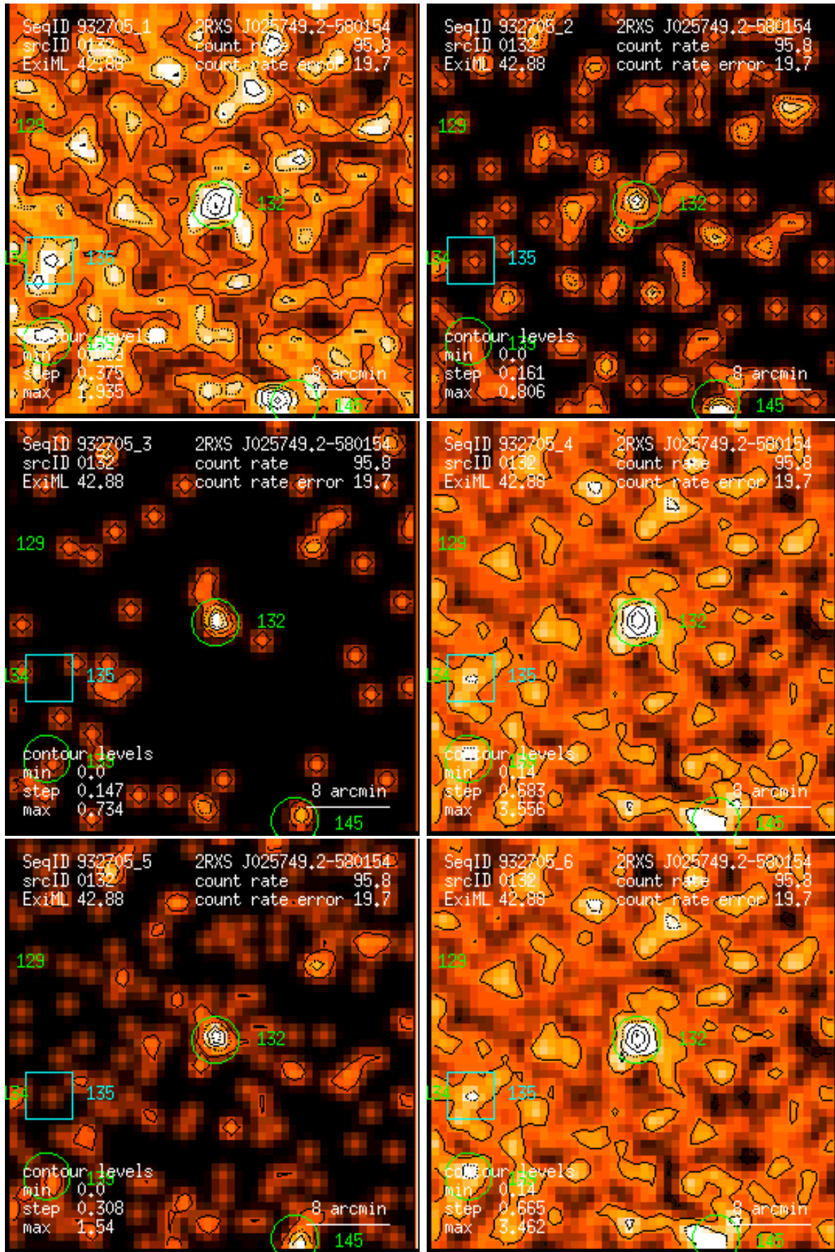
Figure 132: RASS 932705: detection 0132: band rate images, Gaussian filter: (1) PSPC channels 11 – 41, (2) 52 – 90, (3) 91 – 201, (4) 11 – 235, (5) 52 – 201, (6) 11 – 201. Broad band rates in counts/ks. Band rate contour levels in counts/ks/arcmin 2 .
