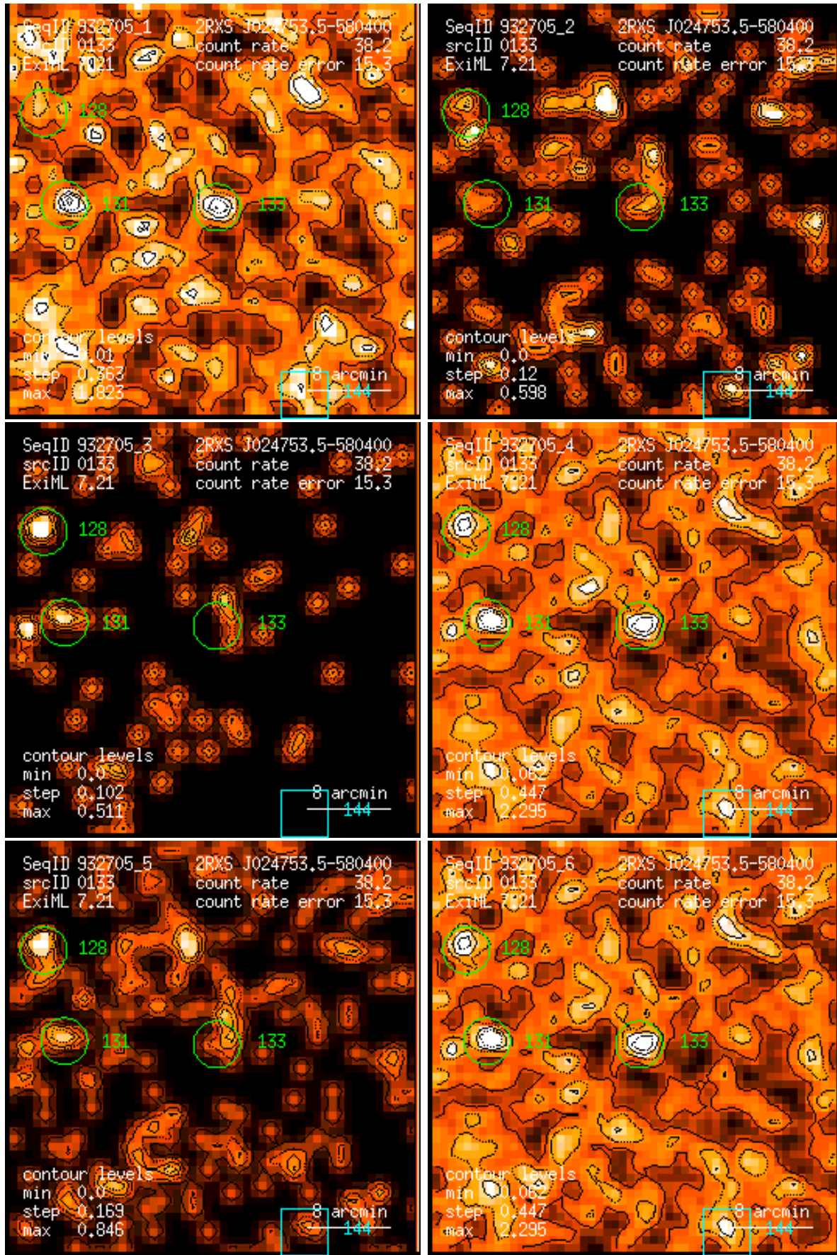
Figure 133: RASS 932705: detection 0133: band rate images, Gaussian filter: (1) PSPC channels 11 – 41, (2) 52 – 90, (3) 91 – 201, (4) 11 – 235, (5) 52 – 201, (6) 11 – 201. Broad band rates in counts/ks. Band rate contour levels in counts/ks/arcmin 2 .
