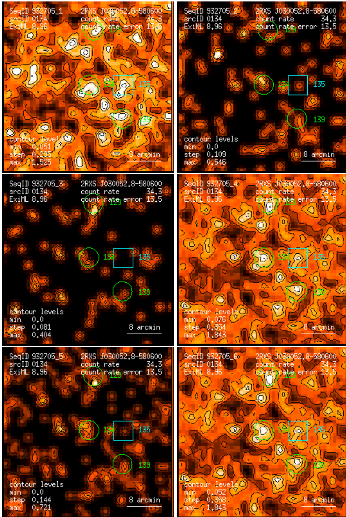
Figure 134: RASS 932705: detection 0134: band rate images, Gaussian filter: (1) PSPC channels 11 – 41, (2) 52 – 90, (3) 91 – 201, (4) 11 – 235, (5) 52 – 201, (6) 11 – 201. Broad band rates in counts/ks. Band rate contour levels in counts/ks/arcmin 2 .
