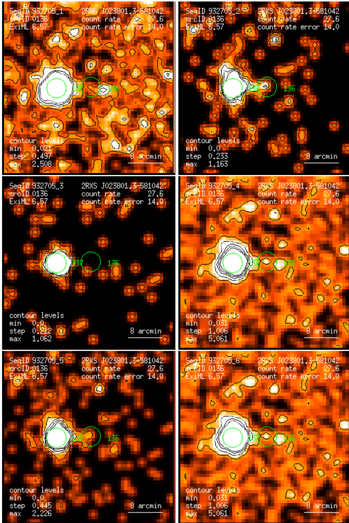
Figure 136: RASS 932705: detection 0136: band rate images, Gaussian filter: (1) PSPC channels 11 – 41, (2) 52 – 90, (3) 91 – 201, (4) 11 – 235, (5) 52 – 201, (6) 11 – 201. Broad band rates in counts/ks. Band rate contour levels in counts/ks/arcmin 2 .
