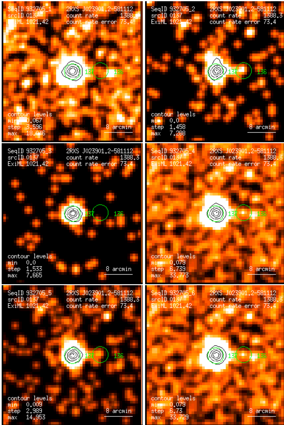
Figure 137: RASS 932705: detection 0137: band rate images, Gaussian filter: (1) PSPC channels 11 – 41, (2) 52 – 90, (3) 91 – 201, (4) 11 – 235, (5) 52 – 201, (6) 11 – 201. Broad band rates in counts/ks. Band rate contour levels in counts/ks/arcmin 2 .
