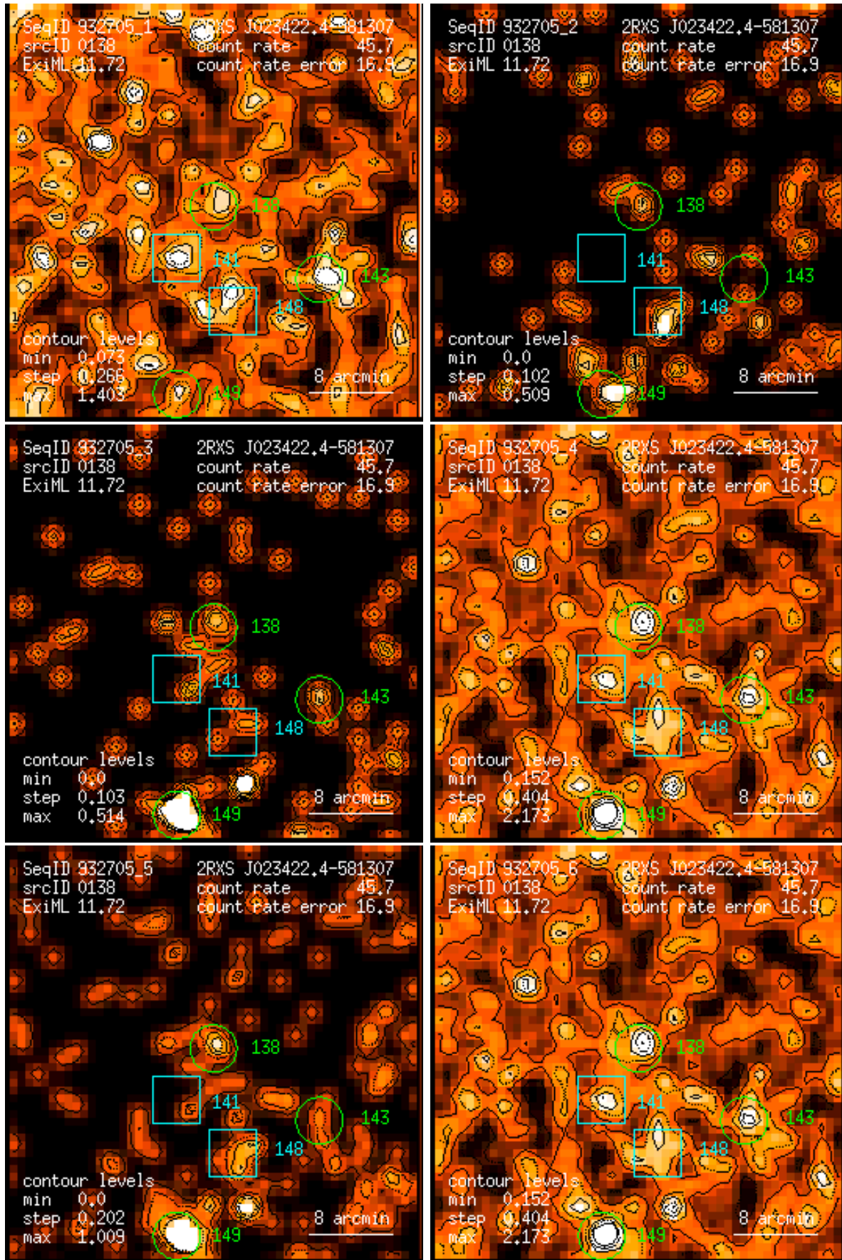
Figure 138: RASS 932705: detection 0138: band rate images, Gaussian filter: (1) PSPC channels 11 – 41, (2) 52 – 90, (3) 91 – 201, (4) 11 – 235, (5) 52 – 201, (6) 11 – 201. Broad band rates in counts/ks. Band rate contour levels in counts/ks/arcmin 2 .
