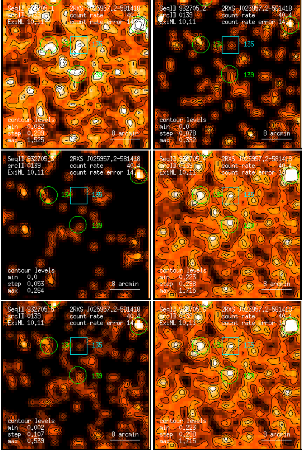
Figure 139: RASS 932705: detection 0139: band rate images, Gaussian filter: (1) PSPC channels 11 – 41, (2) 52 – 90, (3) 91 – 201, (4) 11 – 235, (5) 52 – 201, (6) 11 – 201. Broad band rates in counts/ks. Band rate contour levels in counts/ks/arcmin 2 .
