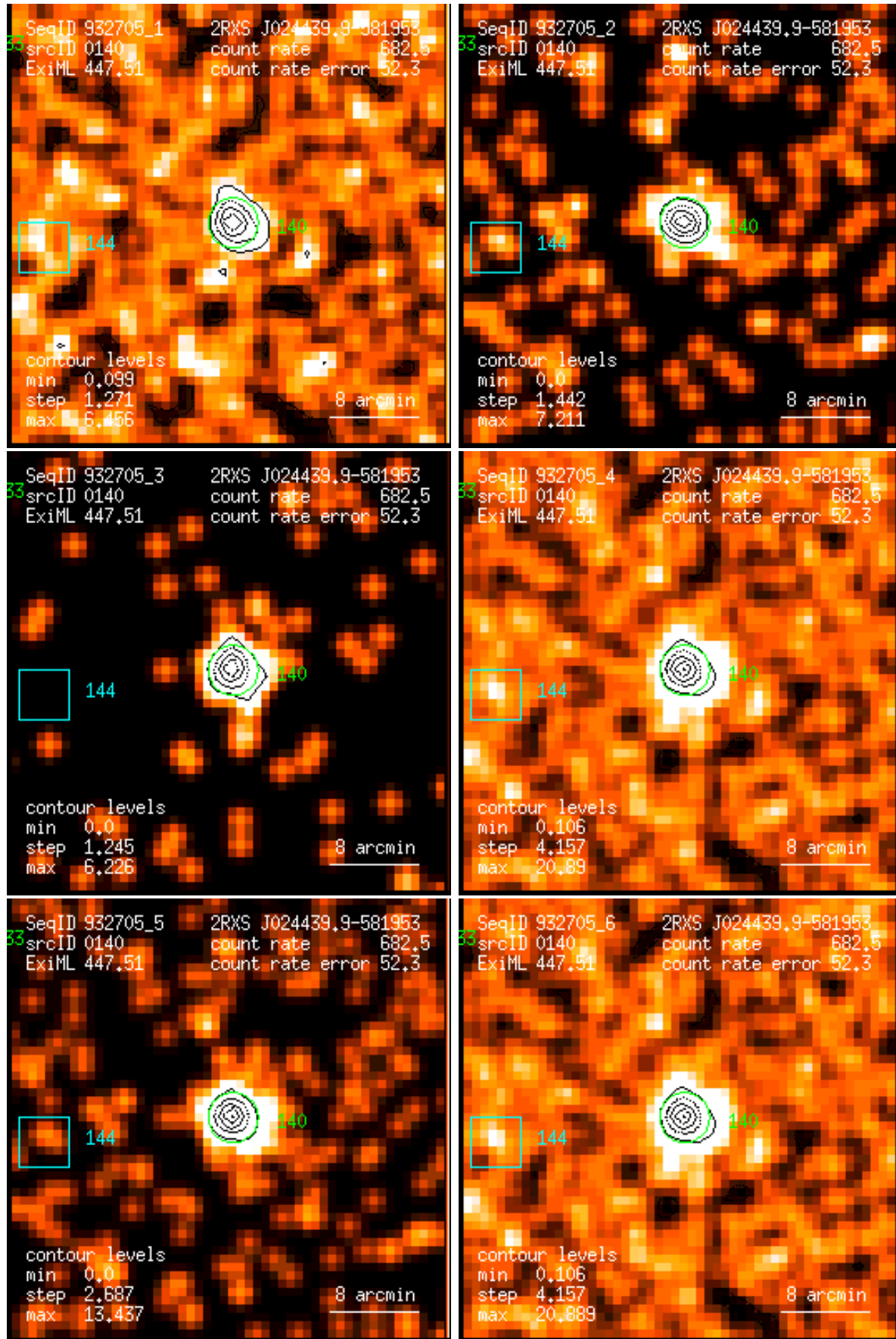
Figure 140: RASS 932705: detection 0140: band rate images, Gaussian filter: (1) PSPC channels 11 – 41, (2) 52 – 90, (3) 91 – 201, (4) 11 – 235, (5) 52 – 201, (6) 11 – 201. Broad band rates in counts/ks. Band rate contour levels in counts/ks/arcmin 2 .
