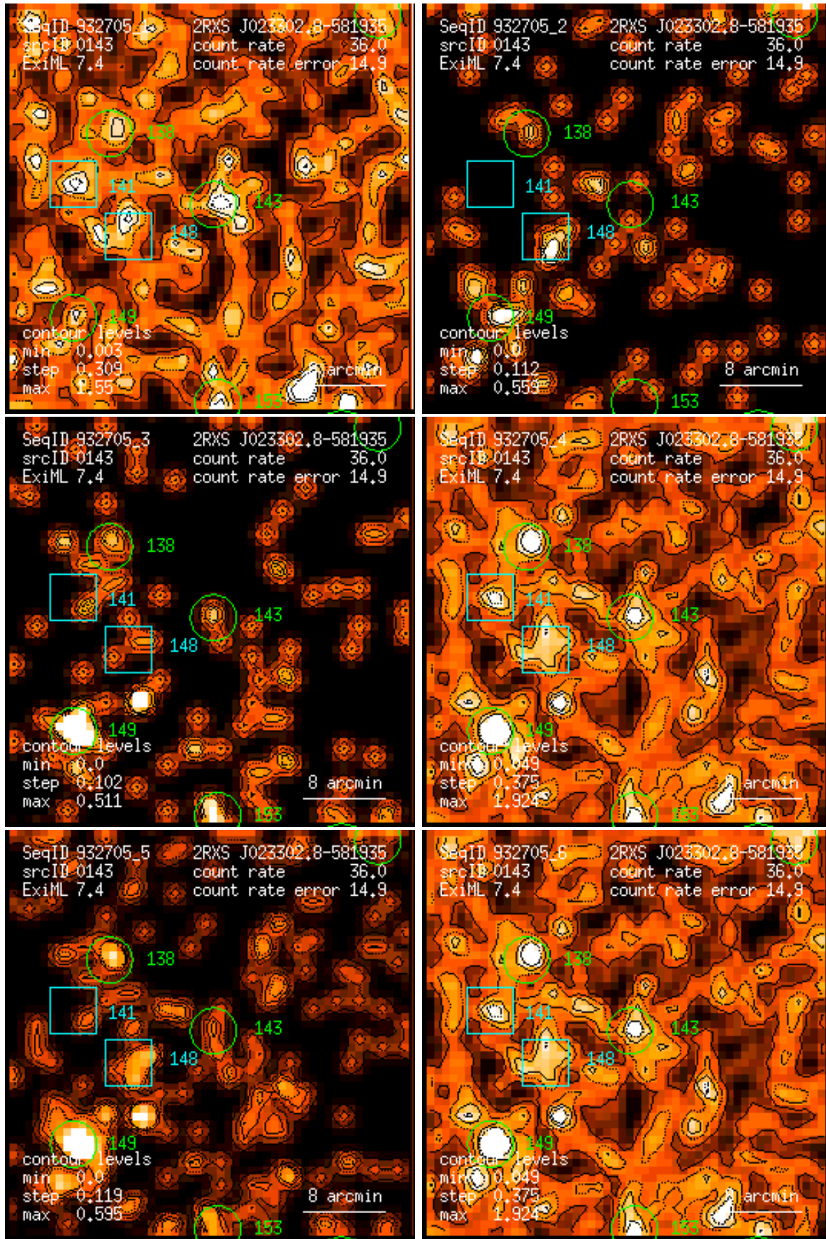
Figure 143: RASS 932705: detection 0143: band rate images, Gaussian filter: (1) PSPC channels 11 – 41, (2) 52 – 90, (3) 91 – 201, (4) 11 – 235, (5) 52 – 201, (6) 11 – 201. Broad band rates in counts/ks. Band rate contour levels in counts/ks/arcmin 2 .
