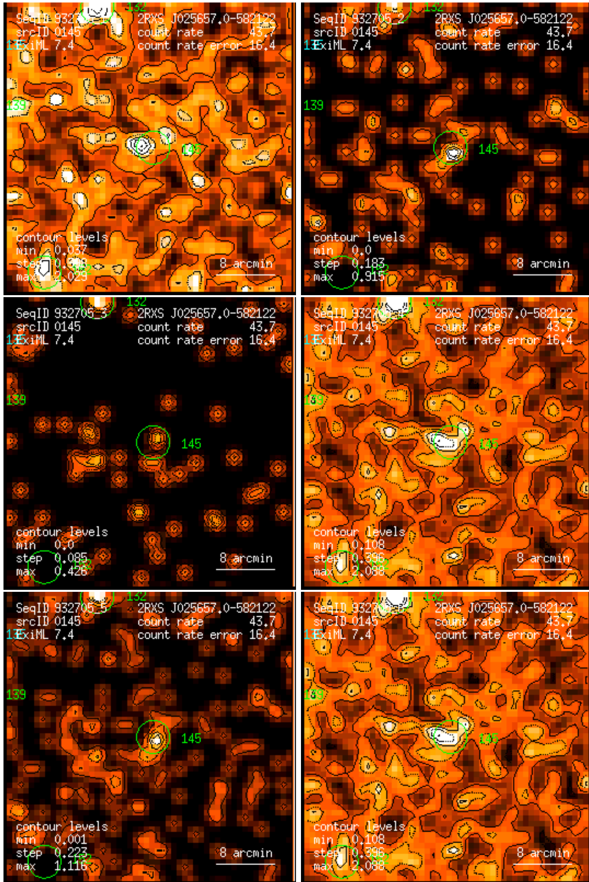
Figure 145: RASS 932705: detection 0145: band rate images, Gaussian filter: (1) PSPC channels 11 – 41, (2) 52 – 90, (3) 91 – 201, (4) 11 – 235, (5) 52 – 201, (6) 11 – 201. Broad band rates in counts/ks. Band rate contour levels in counts/ks/arcmin 2 .
