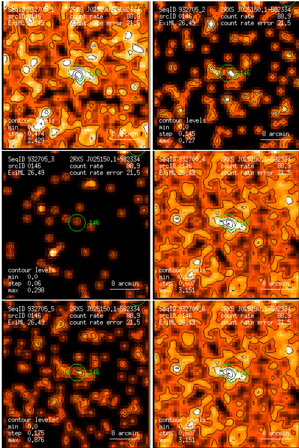
Figure 146: RASS 932705: detection 0146: band rate images, Gaussian filter: (1) PSPC channels 11 – 41, (2) 52 – 90, (3) 91 – 201, (4) 11 – 235, (5) 52 – 201, (6) 11 – 201. Broad band rates in counts/ks. Band rate contour levels in counts/ks/arcmin 2 .
