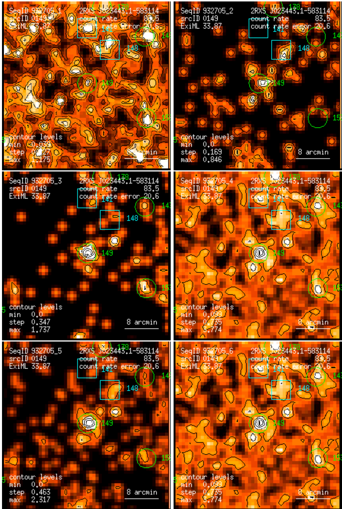
Figure 149: RASS 932705: detection 0149: band rate images, Gaussian filter: (1) PSPC channels 11 – 41, (2) 52 – 90, (3) 91 – 201, (4) 11 – 235, (5) 52 – 201, (6) 11 – 201. Broad band rates in counts/ks. Band rate contour levels in counts/ks/arcmin 2 .
