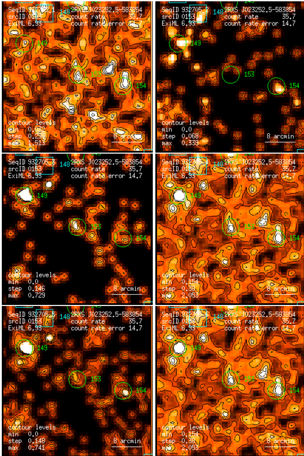
Figure 153: RASS 932705: detection 0153: band rate images, Gaussian filter: (1) PSPC channels 11 – 41, (2) 52 – 90, (3) 91 – 201, (4) 11 – 235, (5) 52 – 201, (6) 11 – 201. Broad band rates in counts/ks. Band rate contour levels in counts/ks/arcmin 2 .
