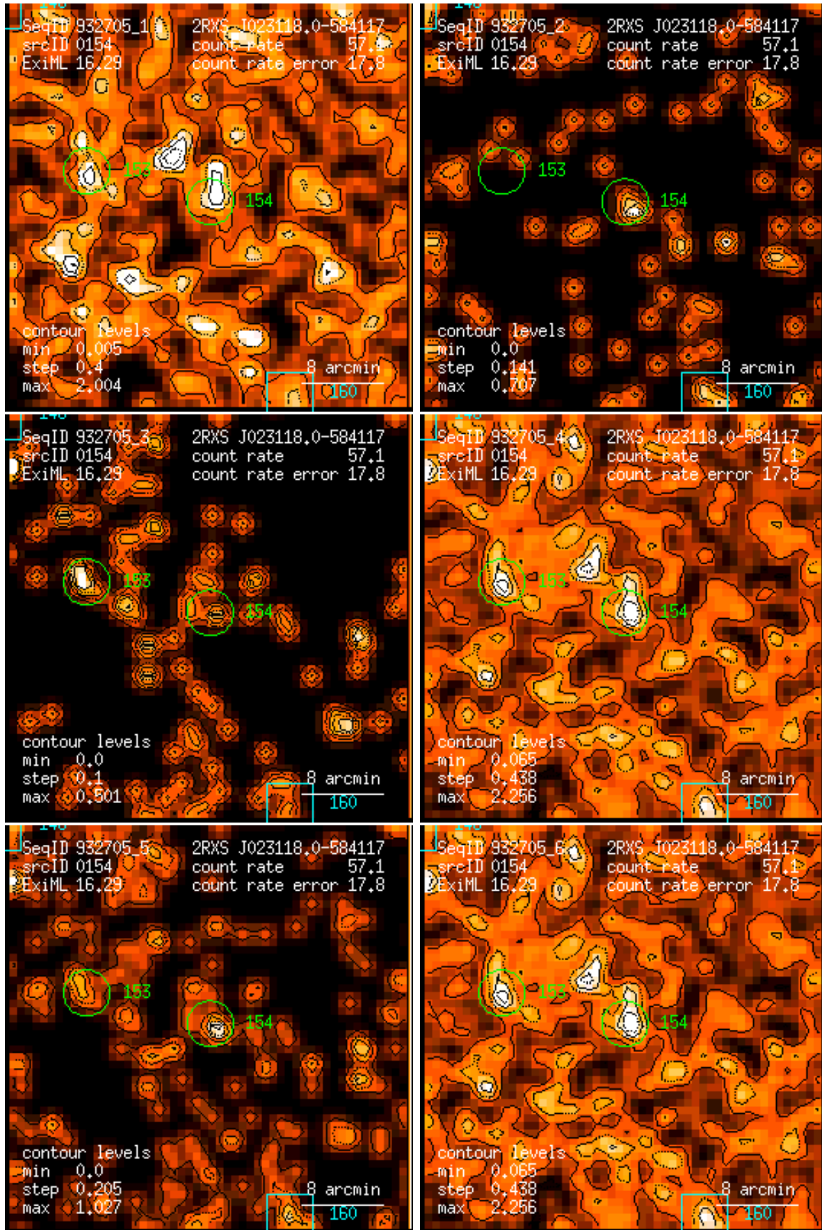
Figure 154: RASS 932705: detection 0154: band rate images, Gaussian filter: (1) PSPC channels 11 – 41, (2) 52 – 90, (3) 91 – 201, (4) 11 – 235, (5) 52 – 201, (6) 11 – 201. Broad band rates in counts/ks. Band rate contour levels in counts/ks/arcmin 2 .
