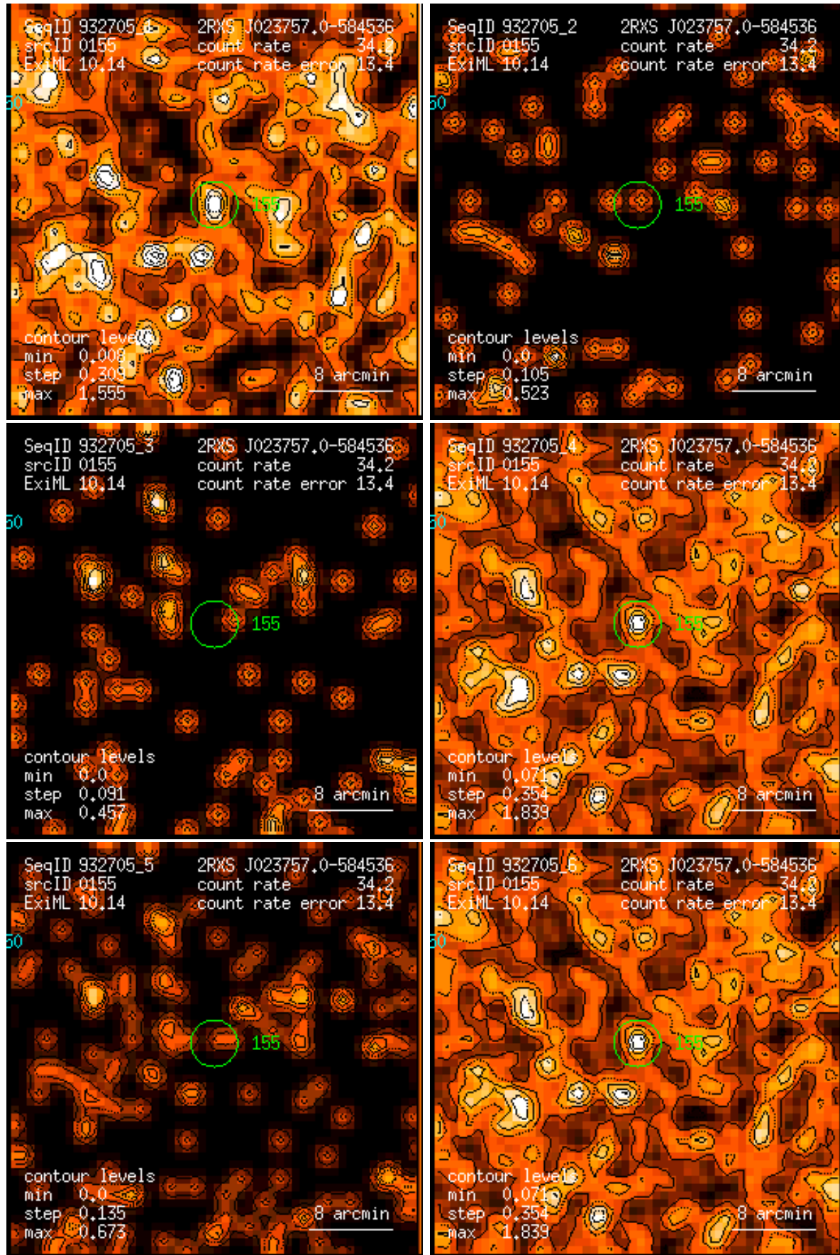
Figure 155: RASS 932705: detection 0155: band rate images, Gaussian filter: (1) PSPC channels 11 – 41, (2) 52 – 90, (3) 91 – 201, (4) 11 – 235, (5) 52 – 201, (6) 11 – 201. Broad band rates in counts/ks. Band rate contour levels in counts/ks/arcmin 2 .
