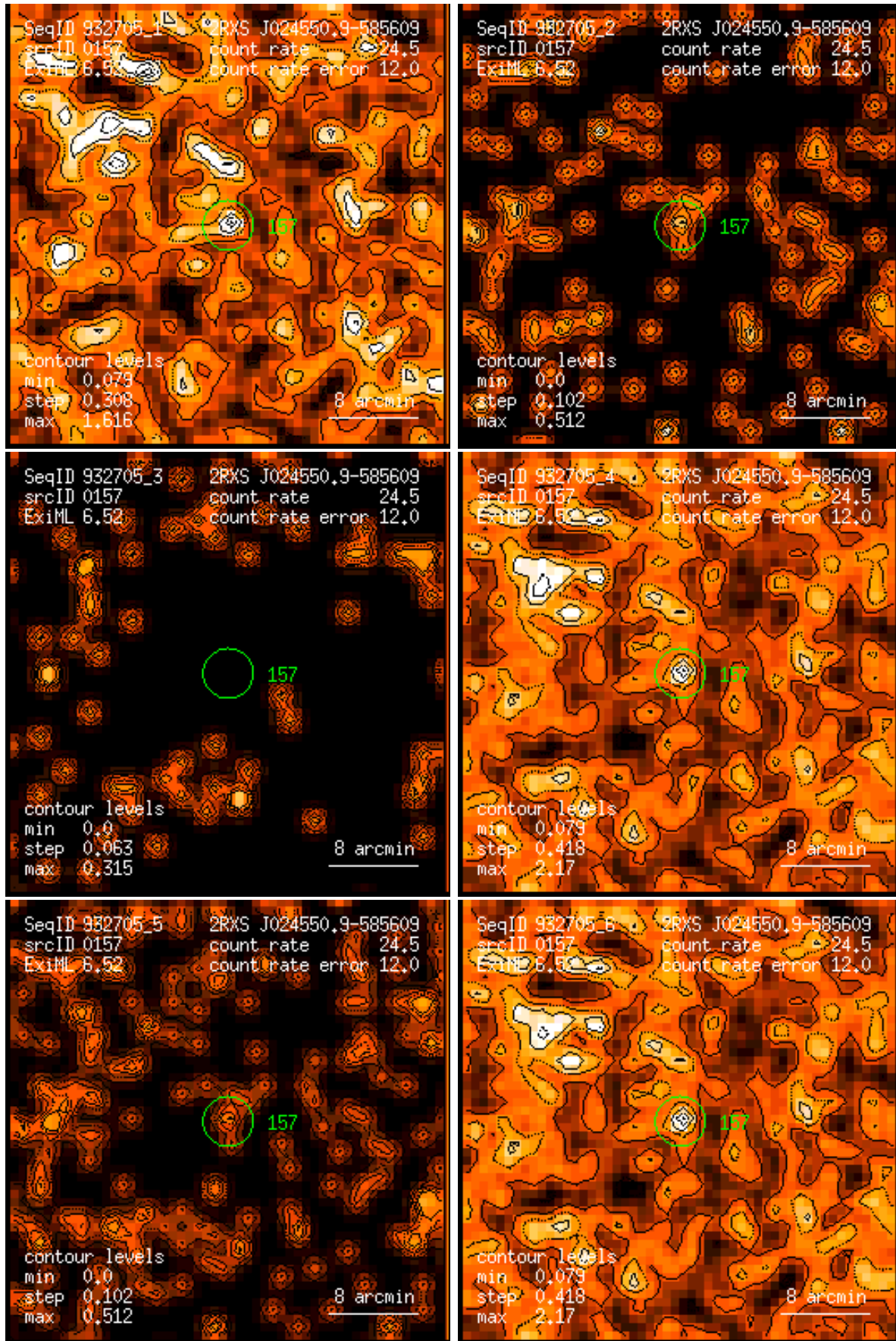
Figure 157: RASS 932705: detection 0157: band rate images, Gaussian filter: (1) PSPC channels 11 – 41, (2) 52 – 90, (3) 91 – 201, (4) 11 – 235, (5) 52 – 201, (6) 11 – 201. Broad band rates in counts/ks. Band rate contour levels in counts/ks/arcmin 2 .
