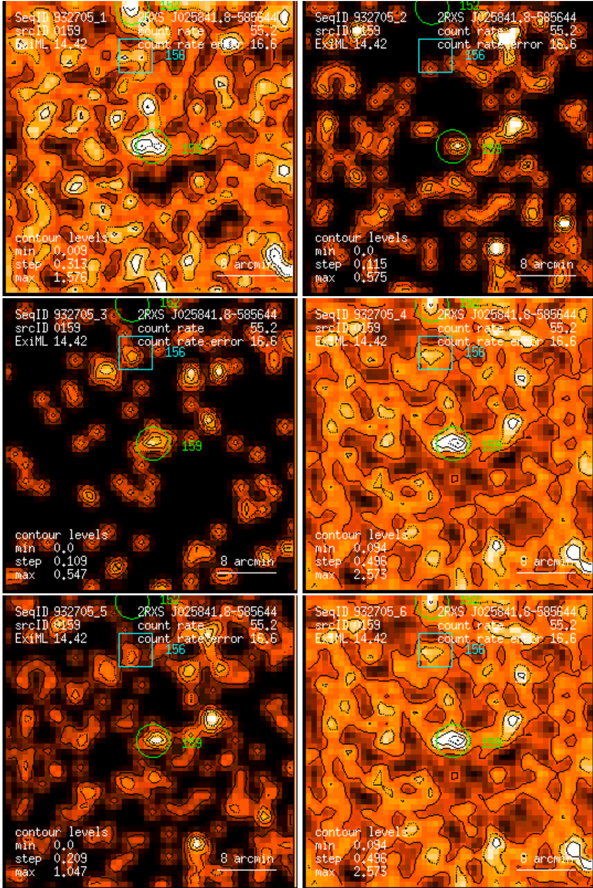
Figure 159: RASS 932705: detection 0159: band rate images, Gaussian filter: (1) PSPC channels 11 – 41, (2) 52 – 90, (3) 91 – 201, (4) 11 – 235, (5) 52 – 201, (6) 11 – 201. Broad band rates in counts/ks. Band rate contour levels in counts/ks/arcmin 2 .
