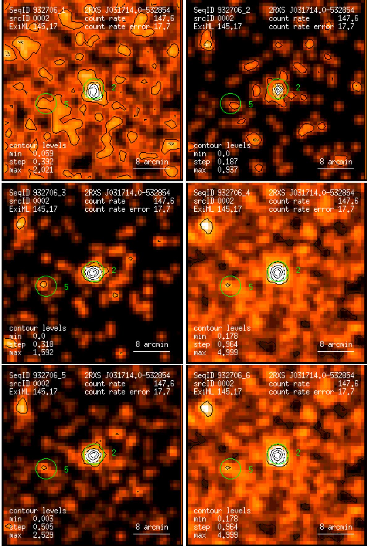
Figure 2: RASS 932706: detection 0002: band rate images, Gaussian filter: (1) PSPC channels 11 – 41, (2) 52 – 90, (3) 91 – 201, (4) 11 – 235, (5) 52 – 201, (6) 11 – 201. Broad band rates in counts/ks. Band rate contour levels in counts/ks/arcmin 2 .
