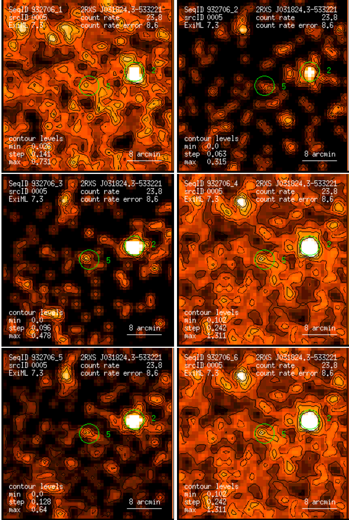
Figure 5: RASS 932706: detection 0005: band rate images, Gaussian filter: (1) PSPC channels 11 – 41, (2) 52 – 90, (3) 91 – 201, (4) 11 – 235, (5) 52 – 201, (6) 11 – 201. Broad band rates in counts/ks. Band rate contour levels in counts/ks/arcmin 2 .
