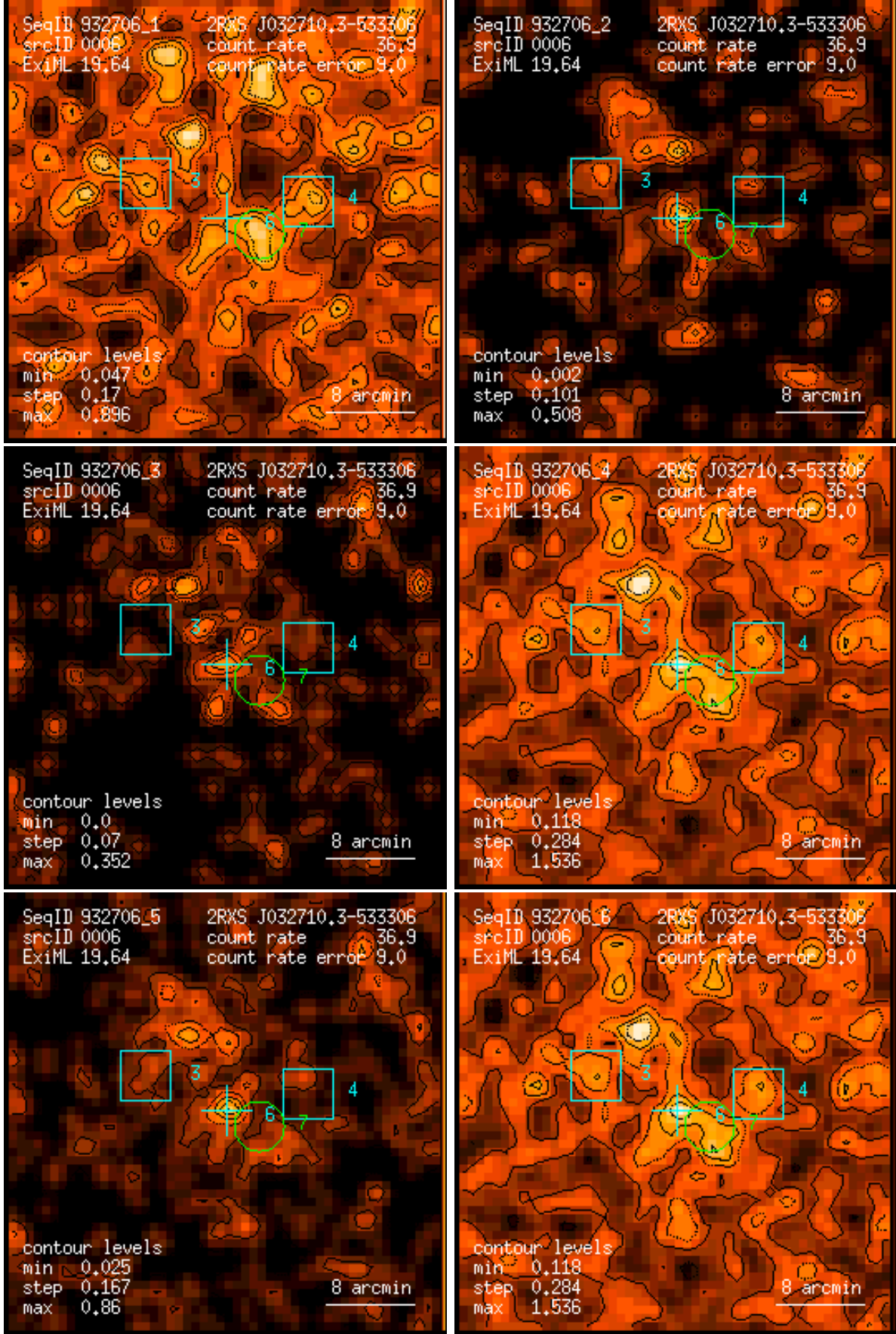
Figure 6: RASS 932706: detection 0006: band rate images, Gaussian filter: (1) PSPC channels 11 – 41, (2) 52 – 90, (3) 91 – 201, (4) 11 – 235, (5) 52 – 201, (6) 11 – 201. Broad band rates in counts/ks. Band rate contour levels in counts/ks/arcmin 2 .
