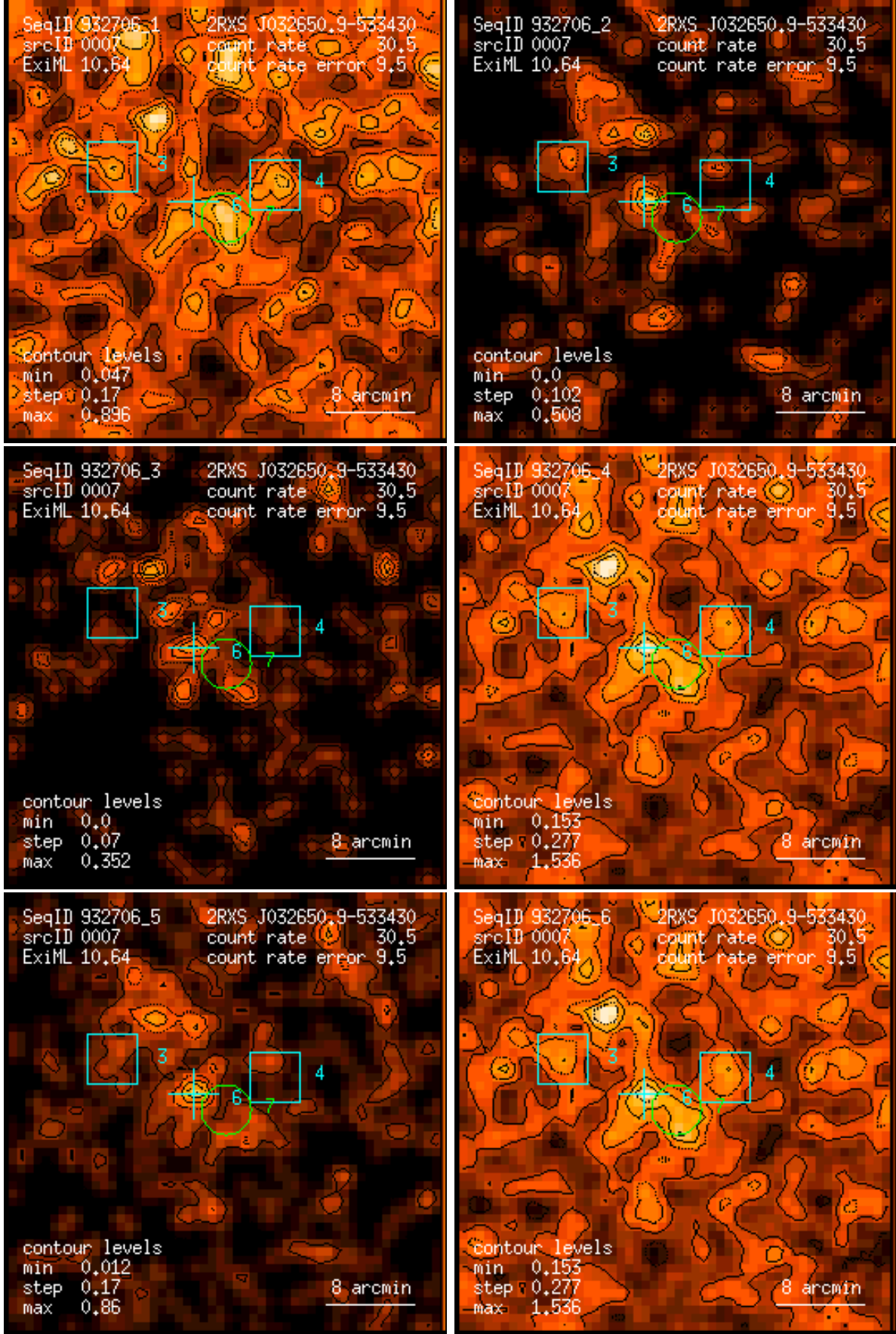
Figure 7: RASS 932706: detection 0007: band rate images, Gaussian filter: (1) PSPC channels 11 – 41, (2) 52 – 90, (3) 91 – 201, (4) 11 – 235, (5) 52 – 201, (6) 11 – 201. Broad band rates in counts/ks. Band rate contour levels in counts/ks/arcmin 2 .
