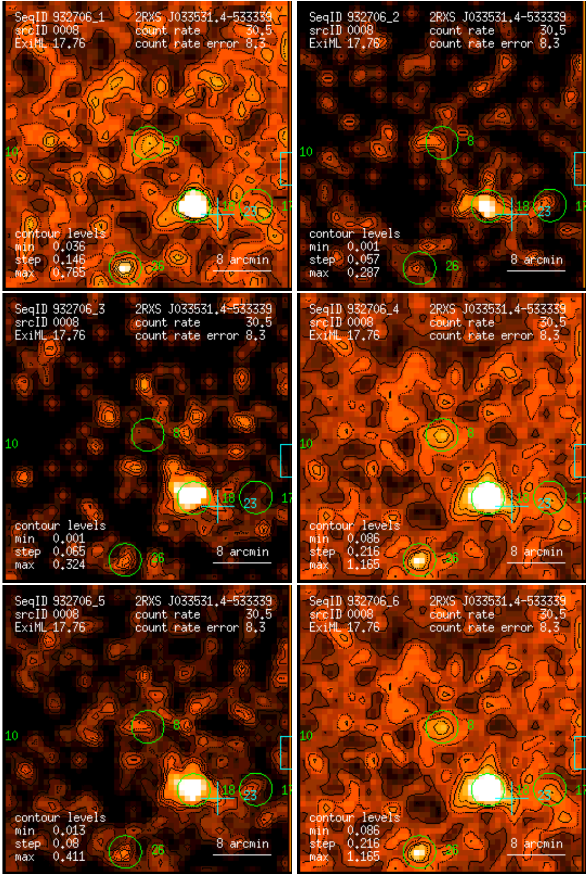
Figure 8: RASS 932706: detection 0008: band rate images, Gaussian filter: (1) PSPC channels 11 – 41, (2) 52 – 90, (3) 91 – 201, (4) 11 – 235, (5) 52 – 201, (6) 11 – 201. Broad band rates in counts/ks. Band rate contour levels in counts/ks/arcmin 2 .
