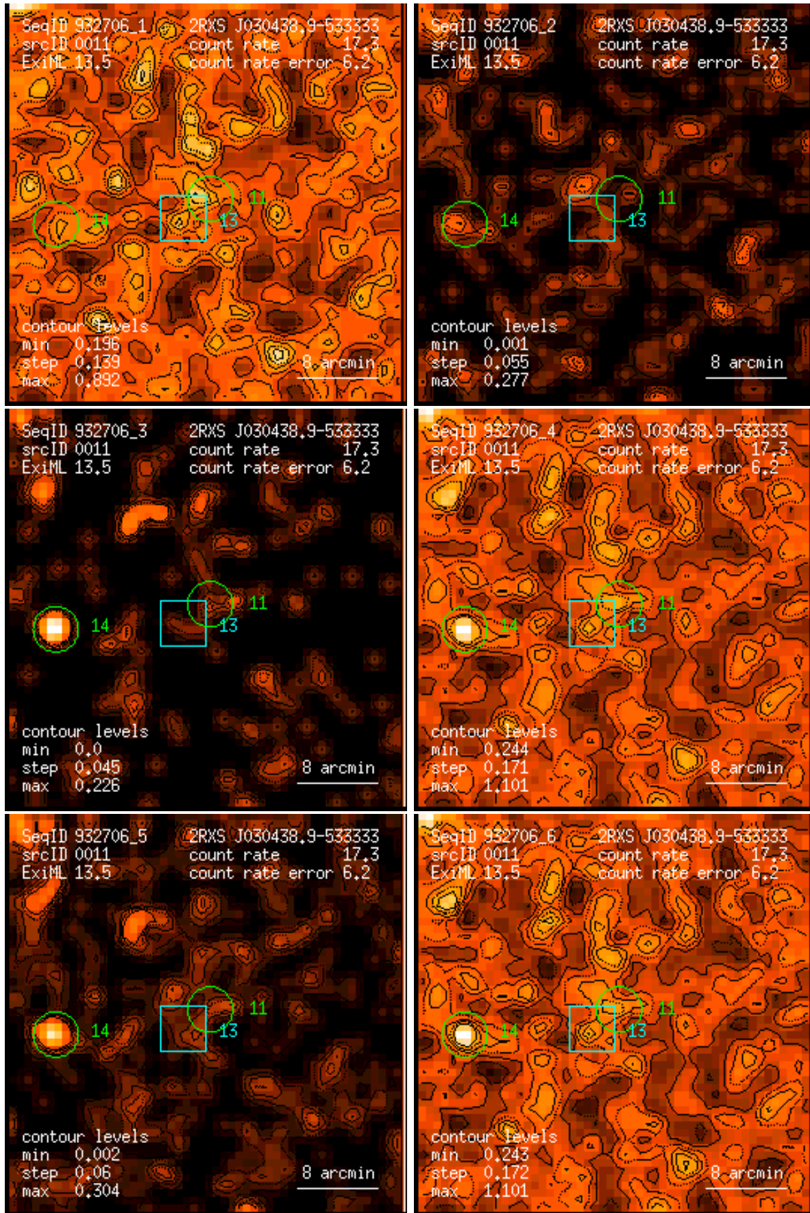
Figure 11: RASS 932706: detection 0011: band rate images, Gaussian filter: (1) PSPC channels 11 – 41, (2) 52 – 90, (3) 91 – 201, (4) 11 – 235, (5) 52 – 201, (6) 11 – 201. Broad band rates in counts/ks. Band rate contour levels in counts/ks/arcmin 2 .
