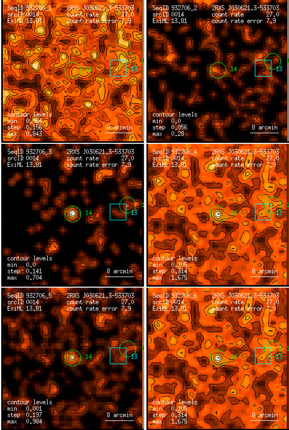
Figure 14: RASS 932706: detection 0014: band rate images, Gaussian filter: (1) PSPC channels 11 – 41, (2) 52 – 90, (3) 91 – 201, (4) 11 – 235, (5) 52 – 201, (6) 11 – 201. Broad band rates in counts/ks. Band rate contour levels in counts/ks/arcmin 2 .
