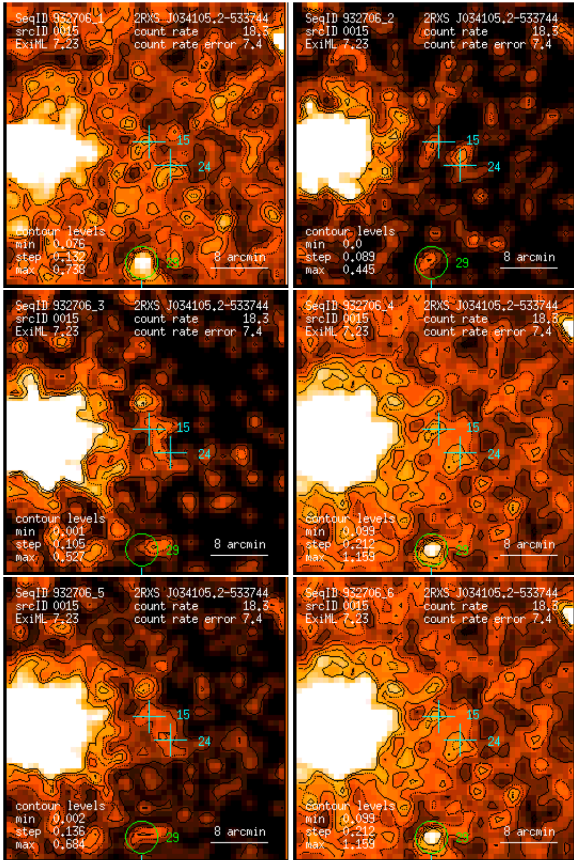
Figure 15: RASS 932706: detection 0015: band rate images, Gaussian filter: (1) PSPC channels 11 – 41, (2) 52 – 90, (3) 91 – 201, (4) 11 – 235, (5) 52 – 201, (6) 11 – 201. Broad band rates in counts/ks. Band rate contour levels in counts/ks/arcmin 2 .
