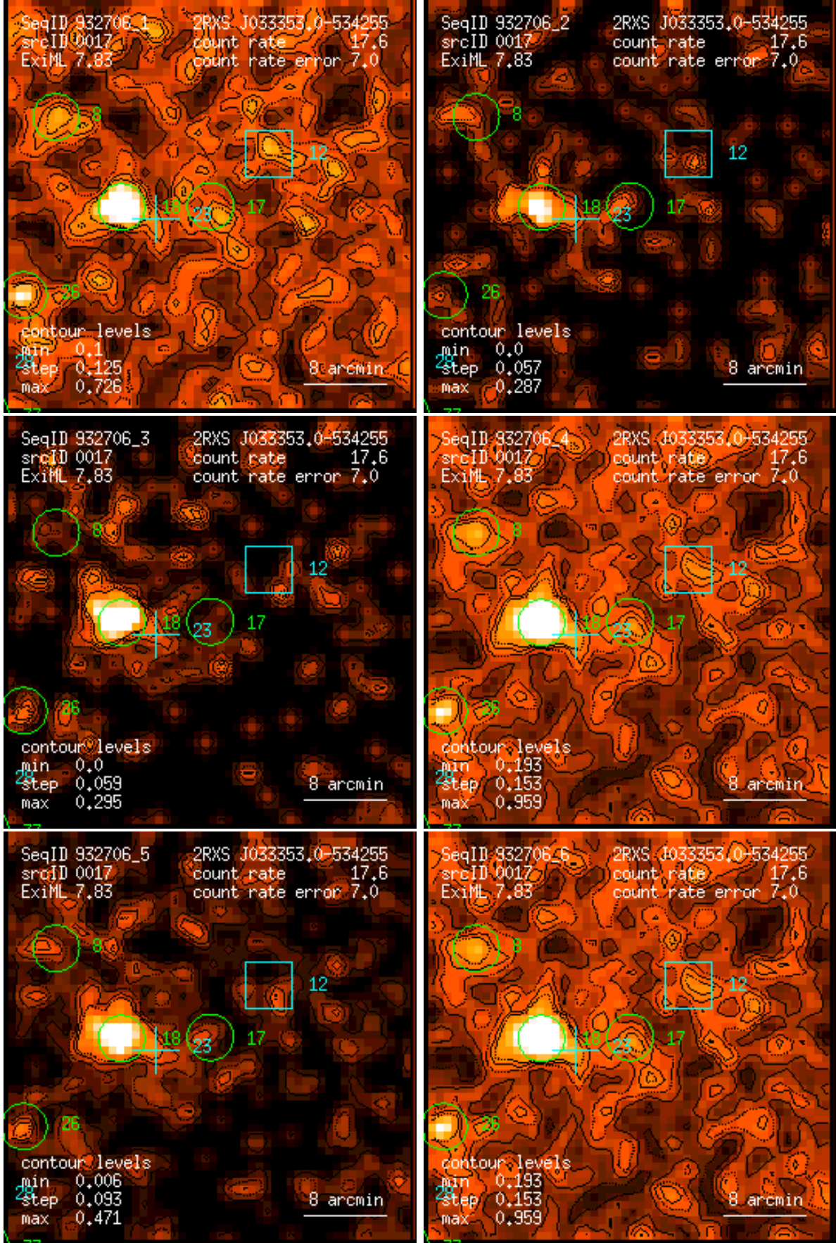
Figure 17: RASS 932706: detection 0017: band rate images, Gaussian filter: (1) PSPC channels 11 – 41, (2) 52 – 90, (3) 91 – 201, (4) 11 – 235, (5) 52 – 201, (6) 11 – 201. Broad band rates in counts/ks. Band rate contour levels in counts/ks/arcmin 2 .
