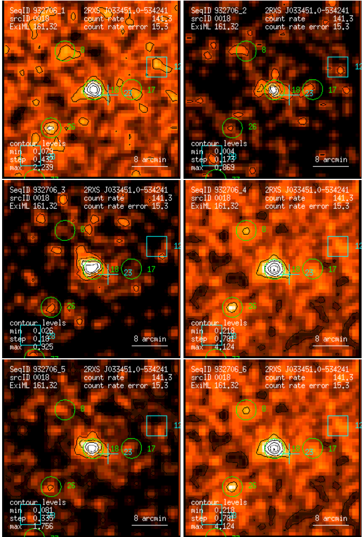
Figure 18: RASS 932706: detection 0018: band rate images, Gaussian filter: (1) PSPC channels 11 – 41, (2) 52 – 90, (3) 91 – 201, (4) 11 – 235, (5) 52 – 201, (6) 11 – 201. Broad band rates in counts/ks. Band rate contour levels in counts/ks/arcmin 2 .
