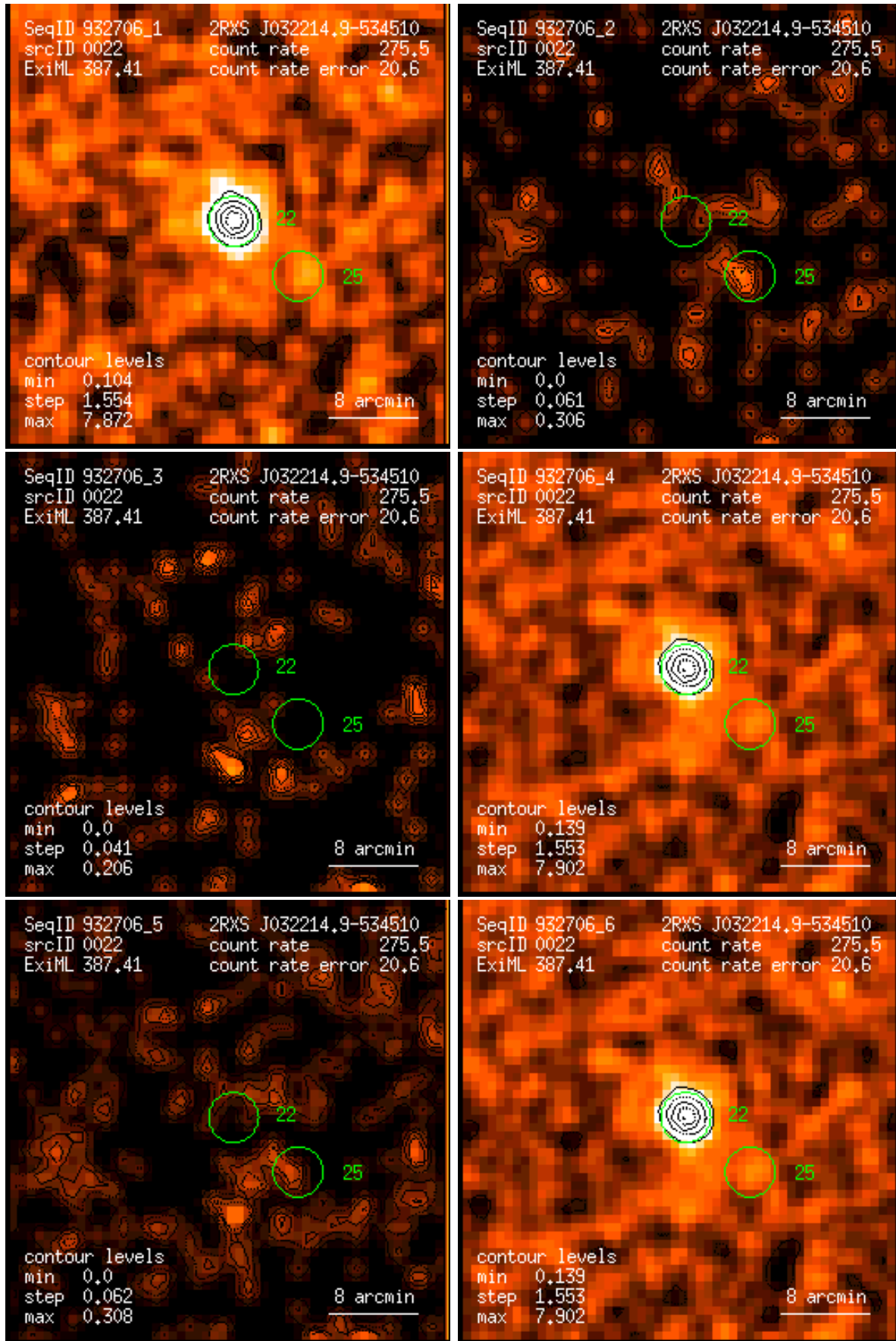
Figure 22: RASS 932706: detection 0022: band rate images, Gaussian filter: (1) PSPC channels 11 – 41, (2) 52 – 90, (3) 91 – 201, (4) 11 – 235, (5) 52 – 201, (6) 11 – 201. Broad band rates in counts/ks. Band rate contour levels in counts/ks/arcmin 2 .
