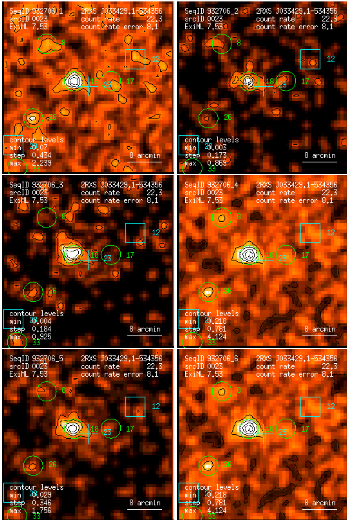
Figure 23: RASS 932706: detection 0023: band rate images, Gaussian filter: (1) PSPC channels 11 – 41, (2) 52 – 90, (3) 91 – 201, (4) 11 – 235, (5) 52 – 201, (6) 11 – 201. Broad band rates in counts/ks. Band rate contour levels in counts/ks/arcmin 2 .
