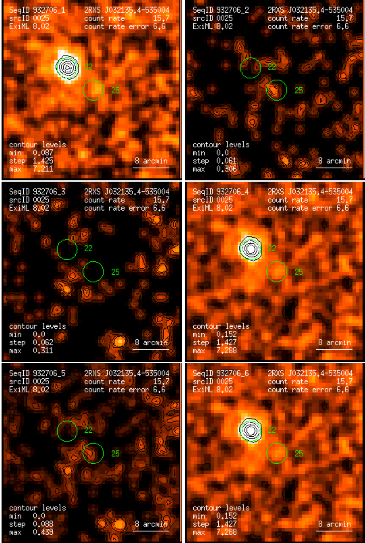
Figure 25: RASS 932706: detection 0025: band rate images, Gaussian filter: (1) PSPC channels 11 – 41, (2) 52 – 90, (3) 91 – 201, (4) 11 – 235, (5) 52 – 201, (6) 11 – 201. Broad band rates in counts/ks. Band rate contour levels in counts/ks/arcmin 2 .
