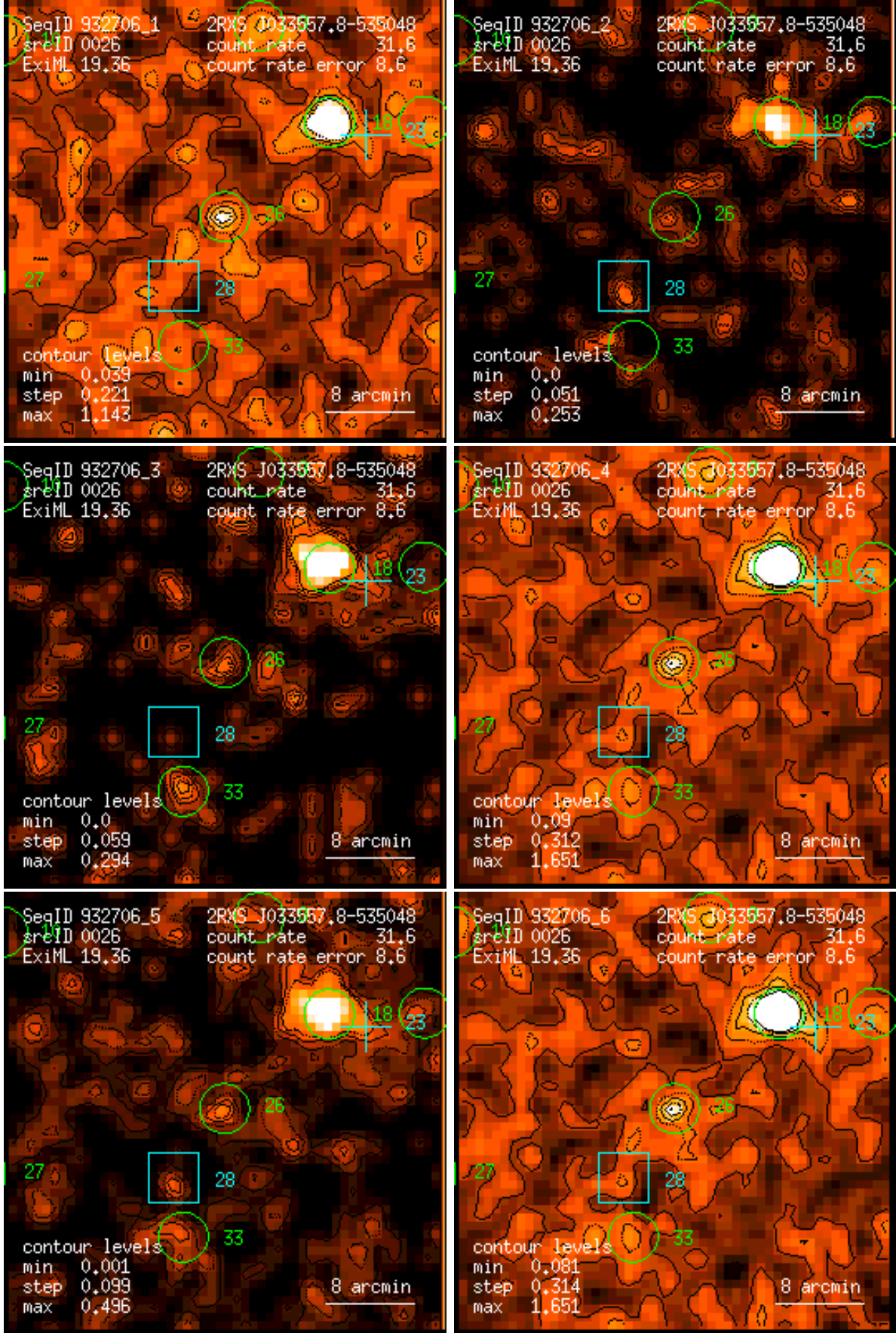
Figure 26: RASS 932706: detection 0026: band rate images, Gaussian filter: (1) PSPC channels 11 – 41, (2) 52 – 90, (3) 91 – 201, (4) 11 – 235, (5) 52 – 201, (6) 11 – 201. Broad band rates in counts/ks. Band rate contour levels in counts/ks/arcmin 2 .
