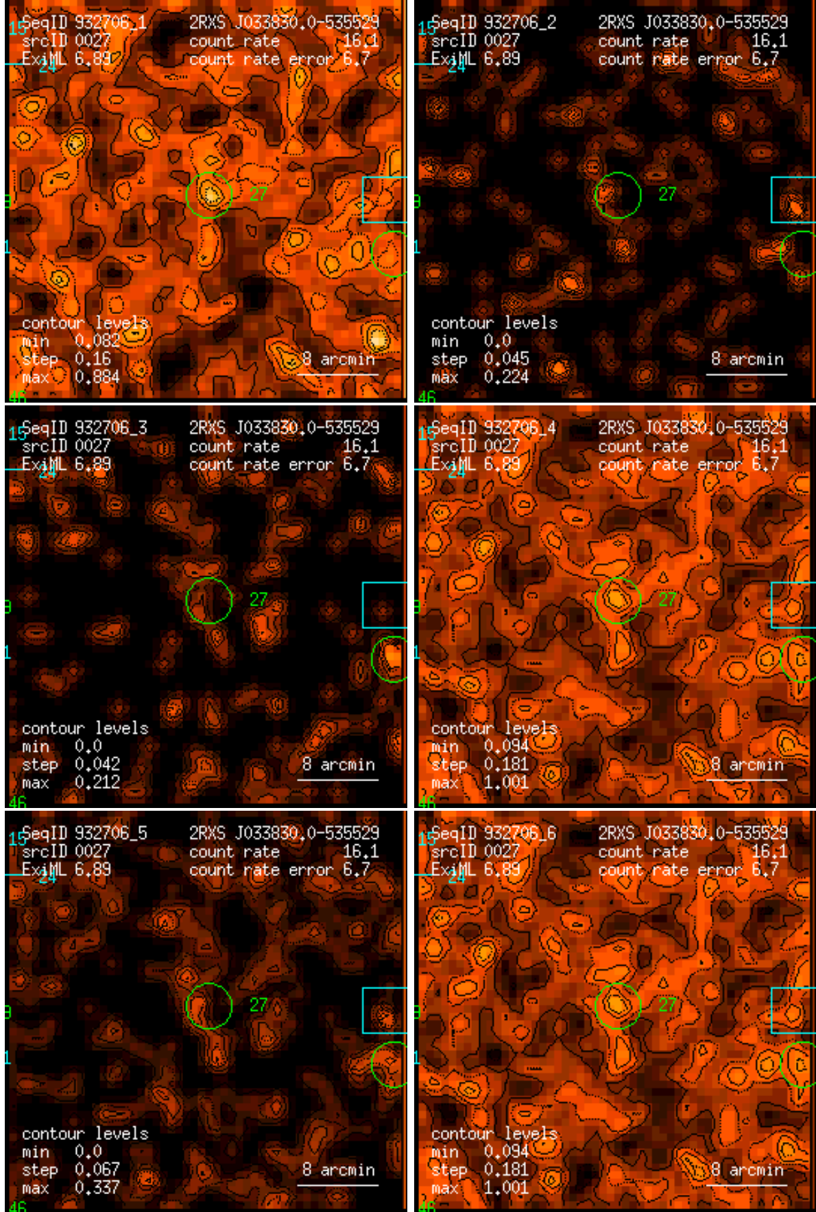
Figure 27: RASS 932706: detection 0027: band rate images, Gaussian filter: (1) PSPC channels 11 – 41, (2) 52 – 90, (3) 91 – 201, (4) 11 – 235, (5) 52 – 201, (6) 11 – 201. Broad band rates in counts/ks. Band rate contour levels in counts/ks/arcmin 2 .
