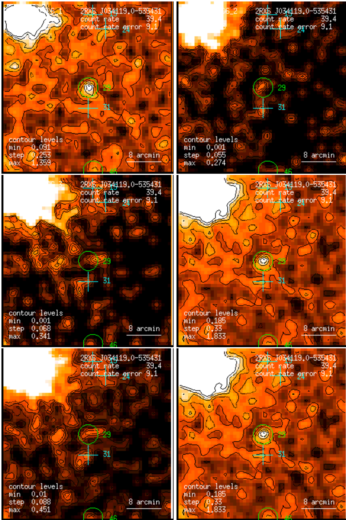
Figure 29: RASS 932706: detection 0029: band rate images, Gaussian filter: (1) PSPC channels 11 – 41, (2) 52 – 90, (3) 91 – 201, (4) 11 – 235, (5) 52 – 201, (6) 11 – 201. Broad band rates in counts/ks. Band rate contour levels in counts/ks/arcmin 2 .
