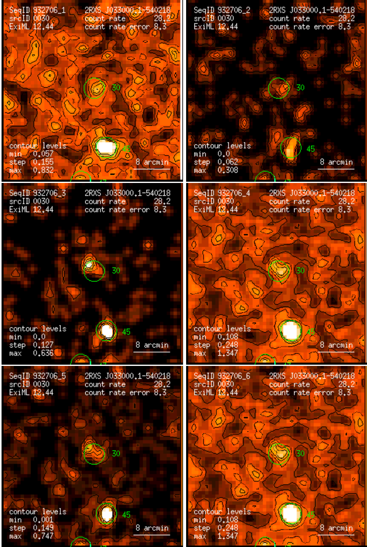
Figure 30: RASS 932706: detection 0030: band rate images, Gaussian filter: (1) PSPC channels 11 – 41, (2) 52 – 90, (3) 91 – 201, (4) 11 – 235, (5) 52 – 201, (6) 11 – 201. Broad band rates in counts/ks. Band rate contour levels in counts/ks/arcmin 2 .
